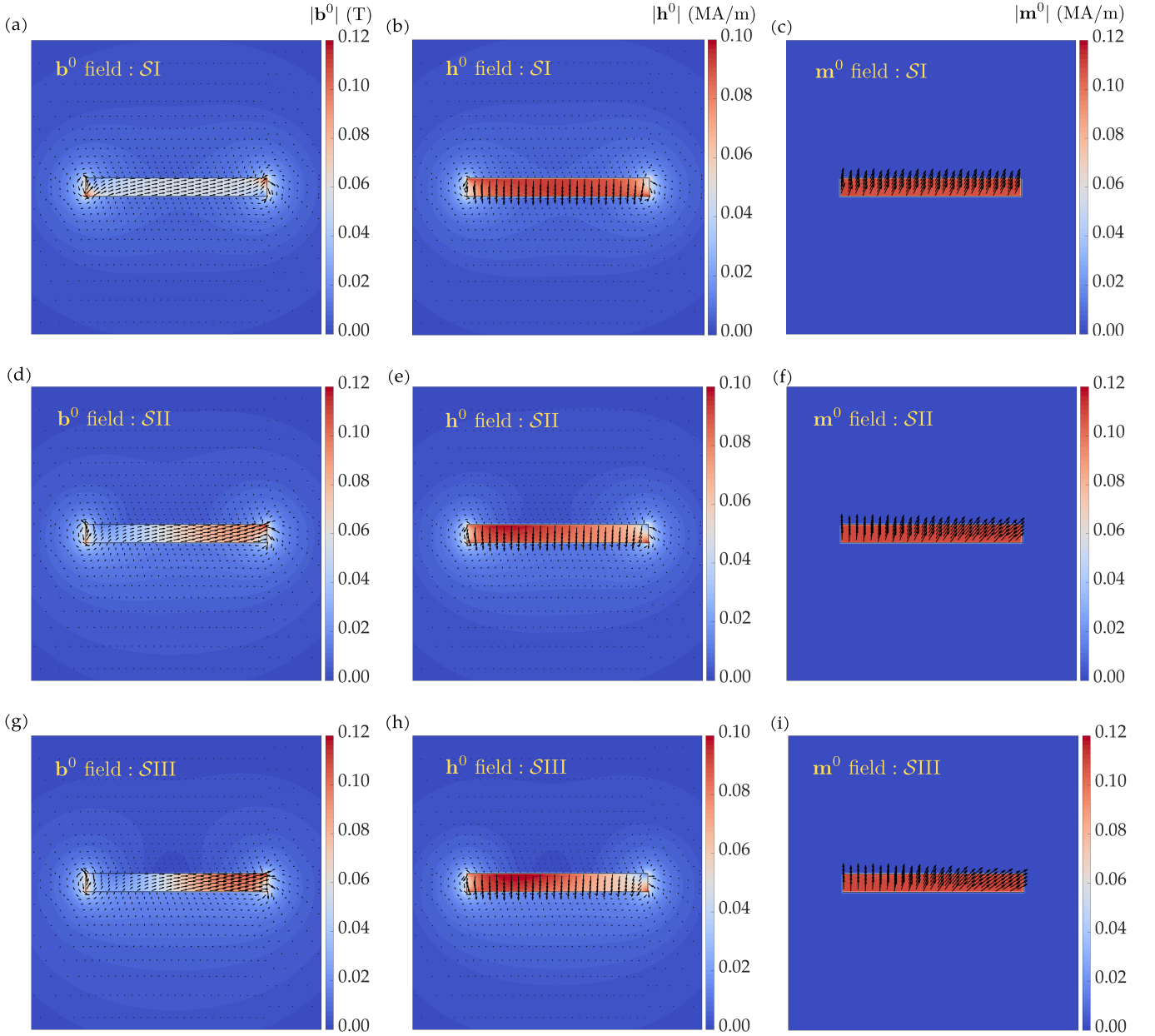
Figure 16: Magnitude and directions of residual \mathbf{b} , \mathbf{h} and \mathbf{m} fields in (a-c) SI, (d-f) SII and (g-i) SIII after the pre-magnetization of the deformed samples along \mathbf{e}_2 (see schematic diagrams in Fig. 15), following a loading path qualitatively similar to Fig. 12b, but having an amplitude of 2 T and after the release of their pre-deformation. The colored contours represent the magnitude of the vector fields, while the black arrows represent their directions.
