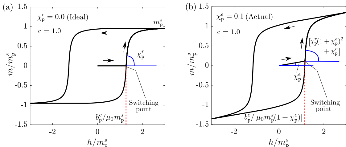
Figure 2: Representative magnetic hysteresis loops. (a) Ideal magnetic particles with no initial magnetization response ( \chi_p^e = 0 ), perfect saturation m_p^s , coercive field b_p^c and the remanent susceptibility \chi_p^r . (b) Actual hard magnetic particles (e.g. NdFeB) with an initial energetic magnetization ( \chi_p^e \neq 0 ) which affects the unloading slope and a very slow saturating response and coercive field b_p^c / (1 + \chi_p^e) . In both cases, the coercive field controls the point where the magnetic switching initiates and is normalized by \mu_0 m_p^s .
