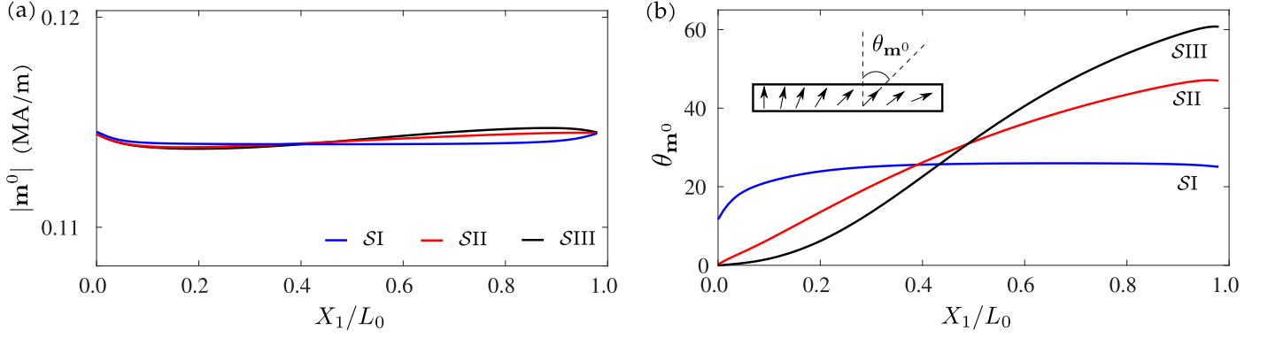
Figure 17: Variation of the residual magnetization \mathbf{m}^0 , induced by the magnetization of the pre-deformed h -MREs, along its length after the pre-deformation is released. The variation of (a) magnitude and (b) direction of the \mathbf{m}^0 vector is shown along the centerline of three differently pre-deformed h -MREs, namely, SI, SII and SIII.
