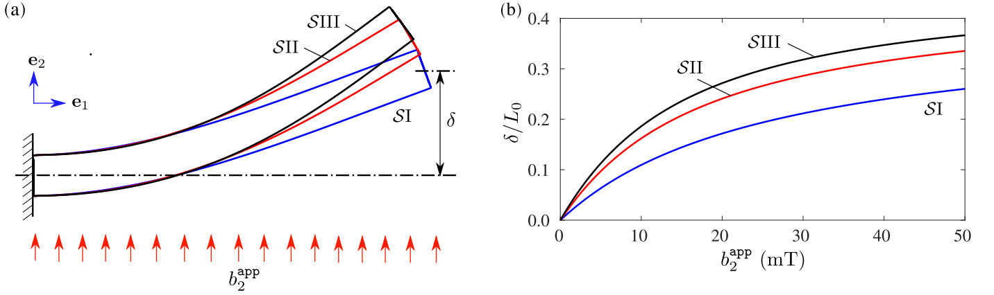
Figure 18: Deflection of non-uniformly magnetized h -MREs SI, SII and SIII under applied field b_2^{\text{app}} having amplitude shown in Fig. 12c and direction along \mathbf{e}_2 . (a) Deflected shapes of SI, SII and SIII under applied b_2^{\text{app}} = 50 mT. (b) Evolutions of the normalized end-tip deflections \delta/L_0 of SI, SII and SIII with b_2^{\text{app}} .
