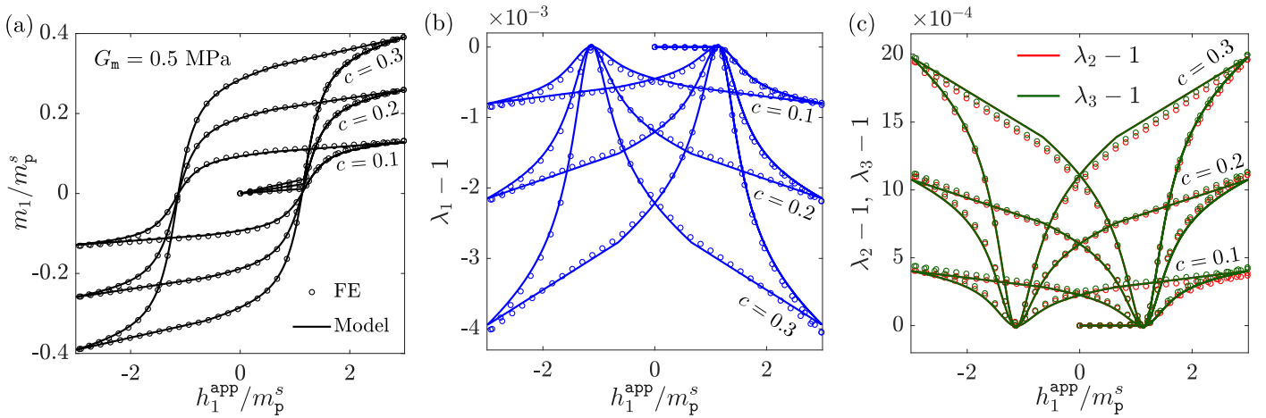
Figure 6: Computed macroscopic hysteresis loops of effective (a) magnetization, (b) parallel and (c) transverse magnetostrictions of h -MRE RVEs having the matrix shear modulus G_m = 0.5 MPa and particle volume fractions c = 0.1, 0.2 and 0.3 . The RVEs are subjected to a fully reversed, proportional cyclic loading having amplitude of 3m_p^s . The average of the effective responses computed from five realizations of a RVE are shown without the fluctuation patches for the magnetostrictions.
