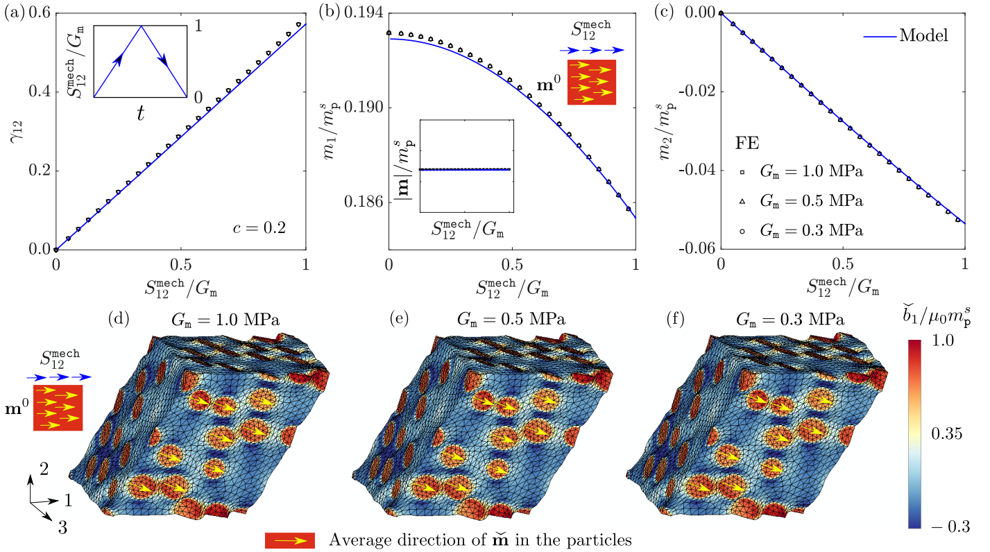
Figure 8: Evolutions of (a) shear strain \gamma_{12} and magnetizations along (b) \mathbf{e}_1 and (c) \mathbf{e}_2 under applied simple shear stress S_{12}^{\text{mech}} , whose loading path is shown in the inset of (a). A schematic of the h -MRE with the direction of pre-magnetization \mathbf{m}^0 and the applied shear stress is shown in the inset of (b). Contours of the \tilde{\mathbf{b}} field in the deformed RVE under applied S_{12}^{\text{mech}}/G_m = 1 for G_m = (d) 1.0, (e) 0.5 and (f) 0.3 MPa. The arrows on the particles show the average direction of \tilde{\mathbf{m}} in them.
