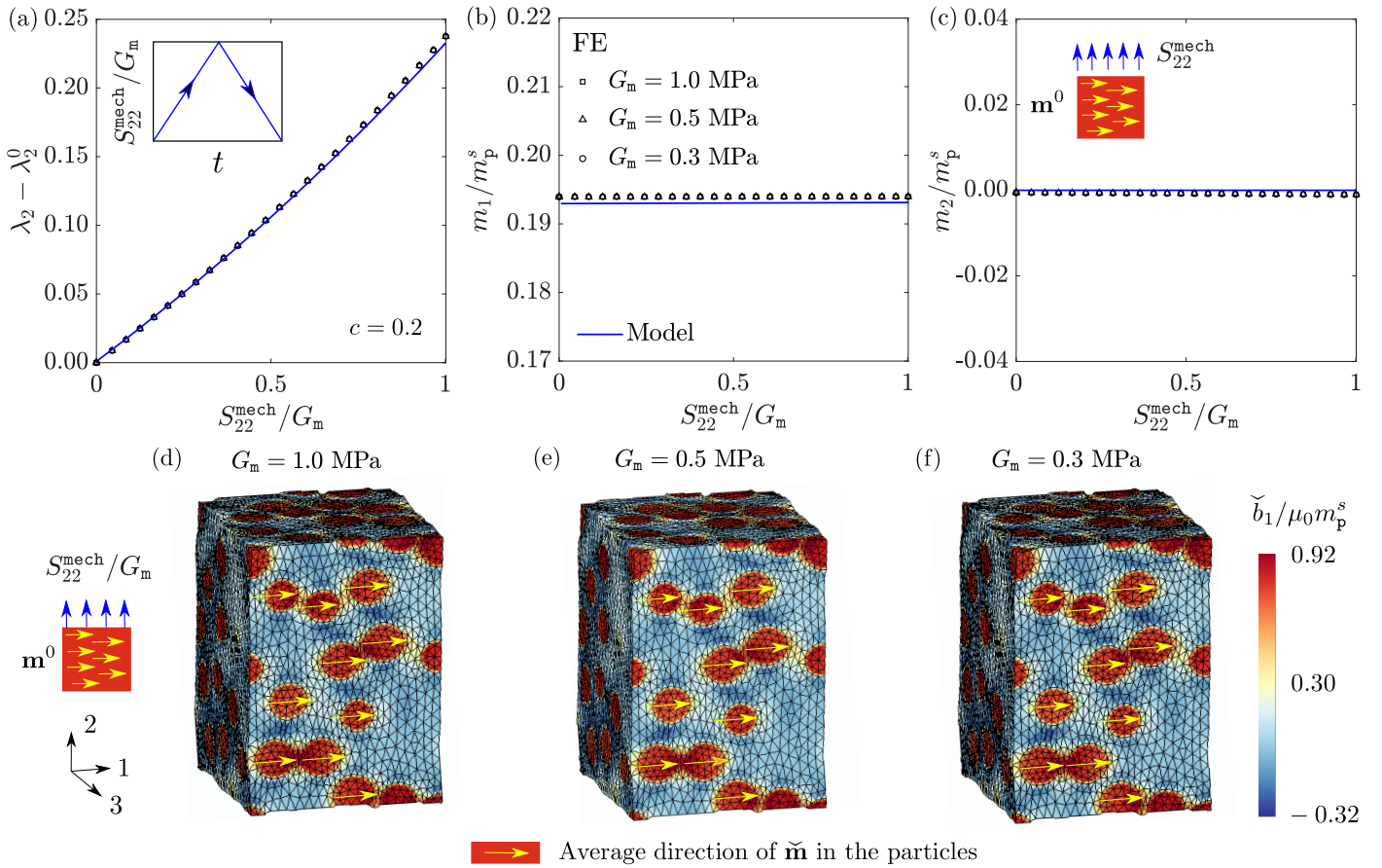
Figure 7: Evolutions of (a) mechanical stretch \lambda_2 - \lambda_2^0 (with \lambda_2^0 denoting the initial remanent stretch due to the pre-magnetization) and magnetizations along (b) \mathbf{e}_1 and (c) \mathbf{e}_2 under applied uniaxial tensile stress S_{22}^{\text{mech}} , whose temporal evolution is shown in the inset of (a). The inset of (c) shows a schematic of the h -MRE with the direction of pre-magnetization \mathbf{m}^0 and the applied uniaxial tension. Contours of the \mathbf{b} field in the deformed RVE under applied S_{22}^{\text{mech}}/G_m = 1 for G_m = (d) 1.0, (e) 0.5 and (f) 0.3 MPa. The arrows on the particles show the average direction of \tilde{\mathbf{m}} in them.
