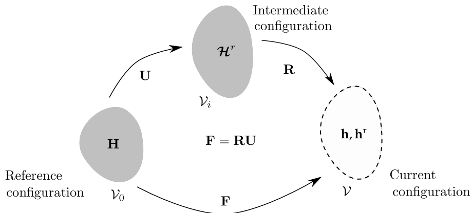
Figure 1: Definition of the independent internal variable \mathcal{H}^r in the intermediate stretch-free configuration \mathcal{V}_i . The components \mathbf{U} and \mathbf{R} denote the stretch tensor and the rotational component, respectively, of the deformation gradient \mathbf{F} .
