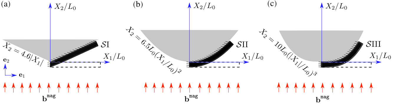
Figure 15: Pre-deformation geometries before the initial magnetization along \mathbf{e}_2 of three different samples of h -MREs, namely (a) SI, (b) SII and (c) SIII, all having the same length L_0 and width w_0 in their undeformed configurations. The pre-magnetizing field \mathbf{b}^{\text{mag}} direction is shown by red arrows, while its magnitude remains the same as in Fig. 12b. The pre-deformed profiles of the top boundary of the h -MREs are given by X_2 = 4.6|X_1| , X_2 = 6.5L_0(X_1/L_0)^2 and X_2 = 10L_0(|X_1/L_0|)^3 for the samples SI, SII and SIII, respectively.
