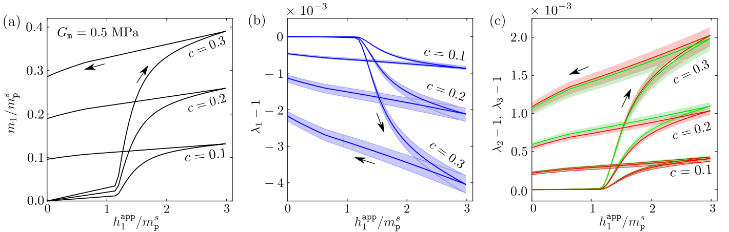
Figure 4: Numerically computed effective (a) magnetization, (b) parallel and (c) transverse magnetostrictions the h -MRE RVEs, subjected to uniaxial Eulerian \mathbf{h}^{\text{app}} = h_1^{\text{app}} \mathbf{e}_1 loading/unloading. The average effective responses (solid lines) along with the range of their fluctuations (light patches) for different realizations of the respective RVEs are indicated. The RVEs of different volume fractions are comprised of random polydisperse spherical hard-magnetic inclusions, coming from three distinct families.
