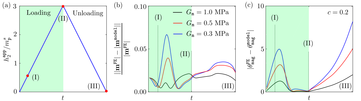
Figure 10: (a) Proportional magnetic loading path along \mathbf{e}_2 , (b) relative difference between the computed and model predicted magnitudes of \mathbf{m} and (c) angle (in an absolute sense) between the computed and the model-predicted effective magnetizations. The points (I), (II) and (III) indicates loading instances at which the deformed RVE along with the b_2 contours are shown in Fig. 11
