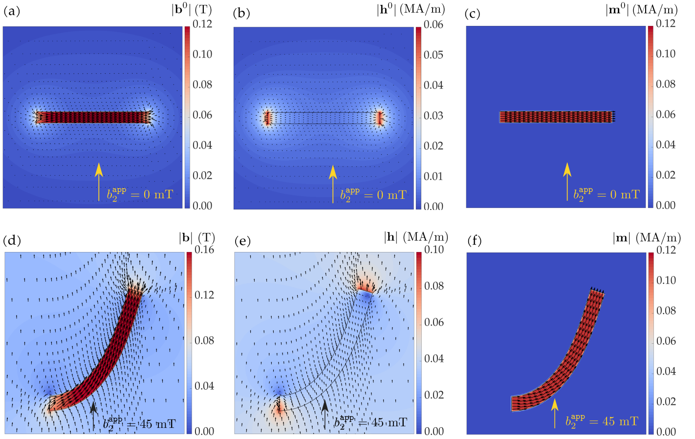
Figure 13: Residual magnetic (a) \mathbf{b} , (b) \mathbf{h} and (c) magnetization \mathbf{m} fields in the h -MRE having an aspect ratio r_{\text{asp}} = 10 , along with magnetic self fields around the surrounding air after Step 1, i.e., the initial magnetization at 2 T. The colored contours represent the magnitude of these fields, whereas the black arrows represent their directions. The lengths of these arrows denote the relative magnitude of the vectors. (d-f) Deflected pre-magnetized h -MRE under an applied transverse field of 45 mT along \mathbf{e}_2 . Magnitude and directions of the resulting (d) \mathbf{b} , (e) \mathbf{h} and (f) \mathbf{m} fields in the h -MRE and its surrounding air is shown by colored contours and black arrows, respectively.
