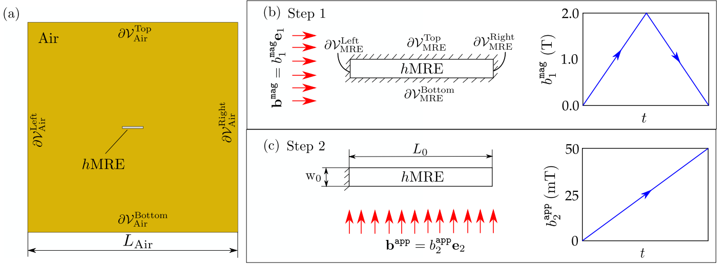
Figure 12: (a) Schematic diagram of the numerical BVP involving the h -MRE and surrounding air. The length of the square air domain L_{\text{Air}} is considered to be L_{\text{Air}} = 10L_0 and four boundaries of this domain are denoted by \partial\mathcal{V}_{\text{Air}}^{\text{Left}} , \partial\mathcal{V}_{\text{Air}}^{\text{Top}} , \partial\mathcal{V}_{\text{Air}}^{\text{Right}} and \partial\mathcal{V}_{\text{Air}}^{\text{Bottom}} . (b) Step 1, indicating the applied pre-magnetizing field \mathbf{b}_1^{\text{mag}} direction (by red arrows) and magnitude (right hand side plot). The four interfaces between air and h -MRE are denoted by \partial\mathcal{V}_{\text{MRE}}^{\text{Left}} , \partial\mathcal{V}_{\text{MRE}}^{\text{Top}} , \partial\mathcal{V}_{\text{MRE}}^{\text{Right}} and \partial\mathcal{V}_{\text{MRE}}^{\text{Bottom}} . The hatched interfaces represent fixed displacement degrees-of-freedom, i.e. \mathbf{u} = \mathbf{0} . (c) Two subsequent magnetic loading paths for (c) Step 2, indicating the actuation field \mathbf{b}_2^{\text{app}} applied along \mathbf{e}_2 , while its magnitude is shown in the adjacent plot. The length and width of the h -MRE are indicated by L_0 and w_0 , respectively, while the fixed h -MRE-air interface in this step is indicated by a hatched line.
