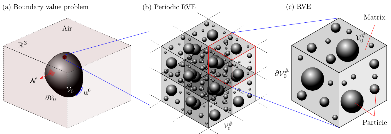
Figure 3: Schematic diagram of (a) macroscopic boundary value problem involving a MRE sample in air having a reference volume \mathcal{V}_0 with unit normal \mathcal{N} on the boundary \partial\mathcal{V}_0 and a representative boundary with fixed displacement \mathbf{u}_0 , (b) periodic arrangement of a RVE with polydisperse spherical inclusions and (c) a RVE occupying a reference volume \mathcal{V}_0^\# and boundary \partial\mathcal{V}_0^\# .
