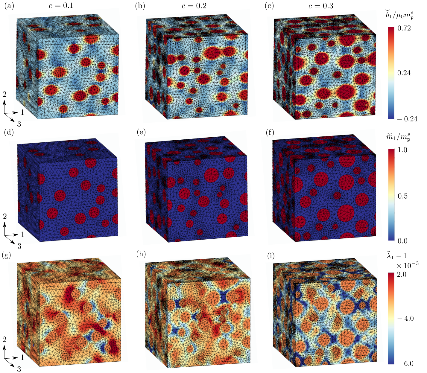
Figure 5: Contours of the numerically computed (a-c) normalized microscopic \tilde{b}_1 , (d-f) normalized local \tilde{m}_1 and (g-i) nominal mechanical strain \tilde{\lambda}_1 - 1 in the RVEs after the first half cycle of loading along \mathbf{e}_1 , under which the effective responses are shown in Fig. 4. Three different, RVEs having (a,d,g) c = 0.1 , (b,e,h) 0.2 and (c,f,i) 0.3 are shown.
