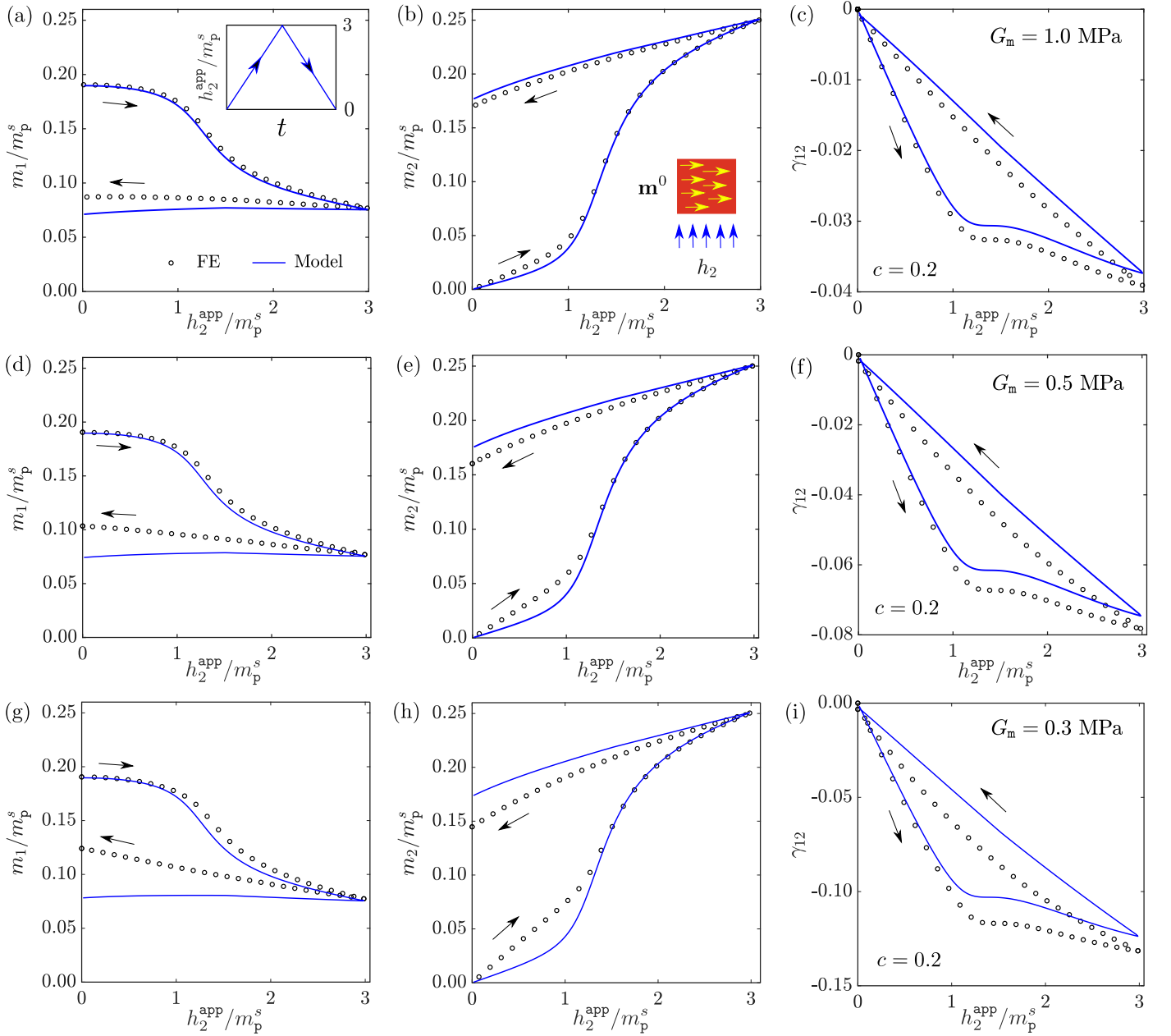
Figure 9: Evolution of the magnetization components along \mathbf{e}_1 (a,d,g) and \mathbf{e}_2 (b,e,h) and the induced shear strain \gamma_{12} (c,f,i) under applied perpendicular magnetic loading along \mathbf{e}_2 (inset of a) to a pre-magnetized h -MRE along \mathbf{e}_1 (inset of b). Effect of three distinct G_m , namely, G_m = (a-c) 1.0 , (d-f) 0.5 and (g-i) 0.3 MPa on the effective magnetization components and induced shear strain.
