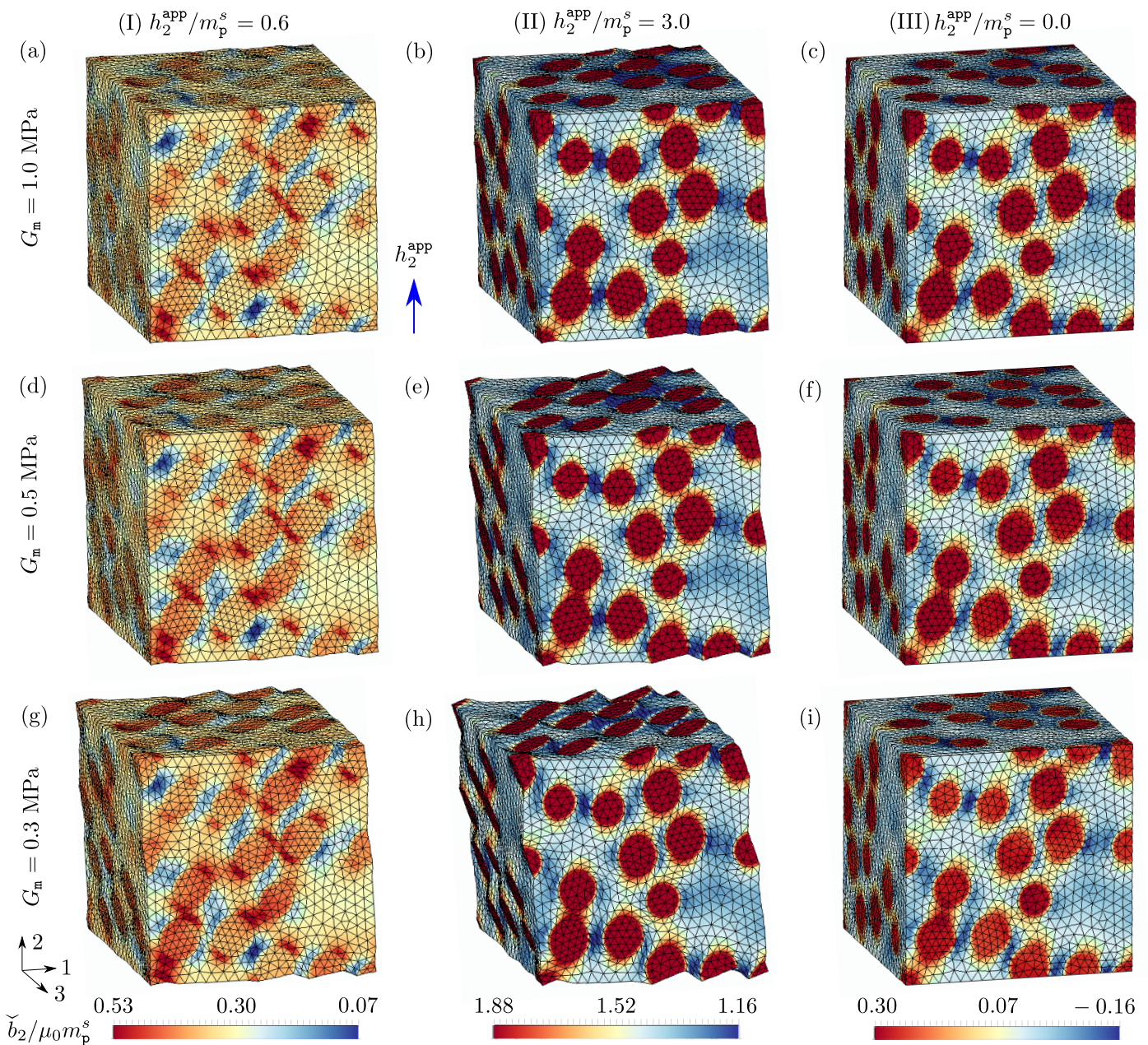
Figure 11: Contours of the numerically computed local \tilde{b}_2 fields in a deformed mesh at the loading/unloading instances (I) (a,d,g), (II) (b,e,h) and (III) (c,f,i) as indicated in Fig. 10a. Contours are shown for three different matrix shear modulus, namely, G_m = 1.0 MPa (a-c), 0.5 MPa (d-f) and 0.3 (g-i).
