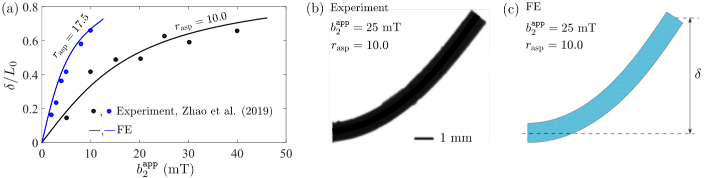
Figure 14: (a) Comparison between numerically computed and experimentally measured end-tip displacement of the pre-magnetized h -MREs (following Steps 1 and 2 as depicted in Fig. 12b and c) having two different aspect ratios r_{\text{asp}} = 10 and 17.5. (b) Experimentally captured deflected beam having r_{\text{asp}} = 10 under b_2^{\text{app}} = 25 mT and (c) numerically computed shape of the pre-magnetized beam of the same r_{\text{asp}} under the same applied b -field.
