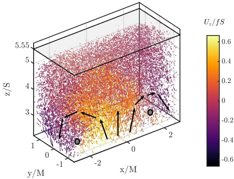
Fig. 4: Example of particle trajectories in a 0.275 s time sample for 25 ppm XG solution. The horizontal shaded rectangle denotes the location of the free surface. Black arrows and grey dots are a guide to the eye respectively illustrating the main flow direction and the center of side vortices.
