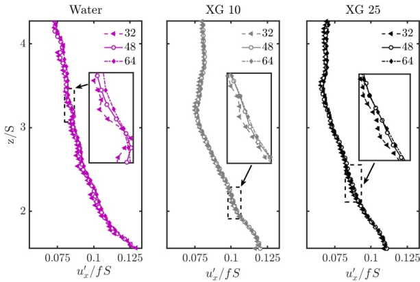
Fig. 5: Influence of spatial resolution (32, 48 or 64 pixel side volumes) of the Eulerian projection on the horizontal turbulence profiles ( u'_x ) scaled by the product fS , for the three working fluids. A zoom insert is associated for each case.
