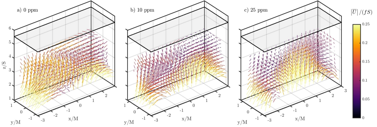
Fig. 8: Mean flow 3D Eulerian velocity fields \bar{U} coloured by the velocity magnitude |\bar{U}| = \sqrt{\bar{U}_x^2 + \bar{U}_y^2 + \bar{U}_z^2} for water (a), C_{XG} = 10 ppm (b) and C_{XG} = 25 ppm (c).
