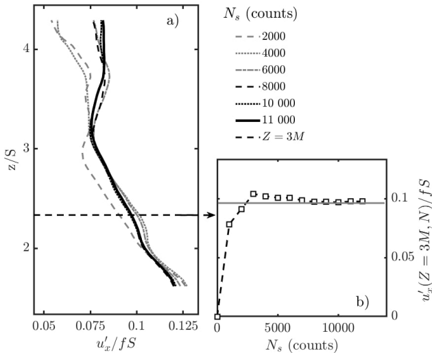
Fig. 6: Statistical convergence of u'_x profiles for the example of the XG10 case. a) Profiles of u'_x/fS versus z/S for various N_s . b) Values of u'_x extracted at z=3M \simeq 2.3S from these profiles and additional ones at other N_s values (not shown in a)), as a function of N_s .
