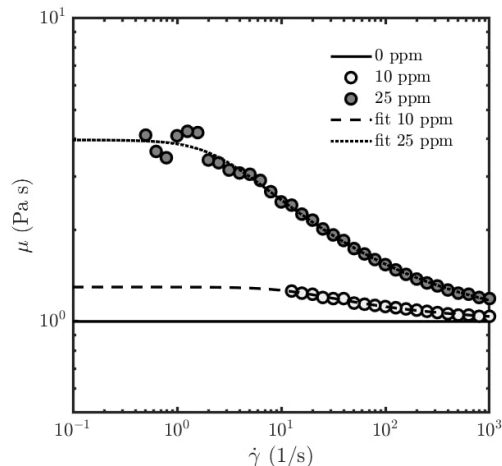
Fig. 2: Viscosity curves and Carreau-Yasuda fitting
