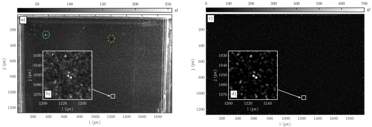
Fig. 3: Example of particle image from camera 1, water run, before (a,b) and after pre-treatment (c,d). b) and d) are zooms of respectively a) and c) on the same group of particles. Dashed circles stress the location of a dust particle crossing the VOI (blue, mixed) and of a shaded spot on the camera sensor (orange, dashed) efficiently removed by the pre-treatment.
