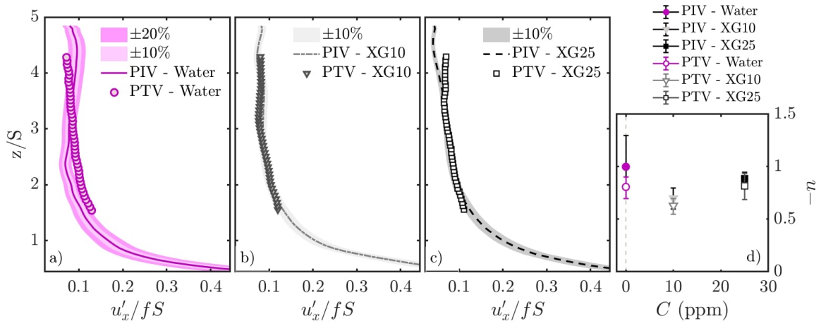
Fig. 9: a,b,c) Width averaged vertical profiles of the RMS of horizontal velocity fluctuations along x ( u'_x ) for the three working fluid considered. Profiles are compared to results obtained by Lacassagne et al (2019b) using PIV. Shaded area correspond to a \pm 10\% uncertainty (and also \pm 20\% for water) around PIV profiles. d) Power law exponents (empty markers) derived from power law fitting of 3D-PTV profiles in (a,b,c). Error bar are 5% confidence intervals on the the fitting parameter. Values and uncertainty reported in Lacassagne et al (2019b) are added for comparison (full markers)
