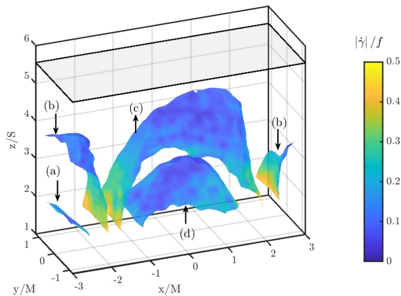
Fig. 10: Isosurface of vertical mean velocity \bar{U}_z scaled by fS at values -0.25 (a), -0.075 (b), 0.075 (c) and 0.25 (d) (XG25 case). Black arrows point the corresponding surface and indicate the vertical velocity direction (up for \bar{U}_z > 0 , down otherwise). The gray rectangle denotes the location of the free surface. Surface are colored by the local shear rate magnitude |\dot{\gamma}| made non dimensional dividing by f .
