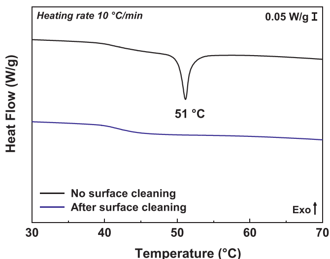
Fig. 9. DSC thermograms (obtained with a heating rate of 10\text{ °C}\cdot\text{min}^{-1} under nitrogen flow) for a Si-g-LLDPE film stabilised with 3.3 wt% of Irganox 1076® before and after its surface cleaning with acetone.
