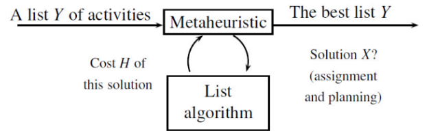
Fig. 1. Hybridisation of a meta-heuristic and a list algorithm
