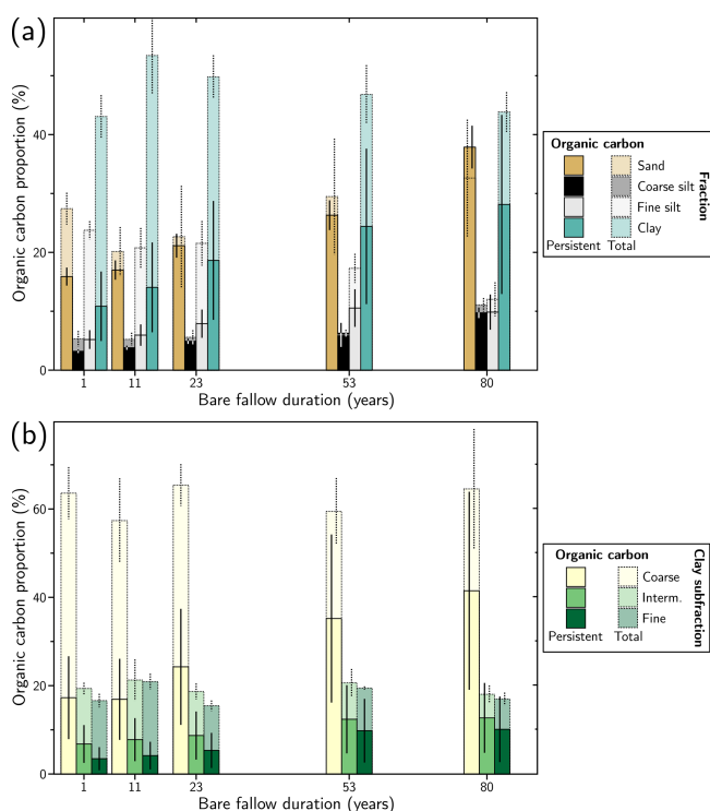
Figure 2. Evolution of the organic carbon proportion contained in the studied size fractions with duration of the LTBF experiment: (a) sand (> 50 μm), silt (coarse: (20–50) μm, fine: (2–20) μm) and clay (< 2 μm) fractions; (b) coarse ((0.2–2) μm), intermediate ((0.05–0.2) μm) and fine (< 0.05 μm) clay subfractions. The error bars, corresponding to 2 standard deviations, are calculated from the standard deviation of the organic carbon content and of the mass of the fraction measured for the four plot replicates. The proportion of persistent organic carbon (dark colour) is obtained from exponential decay fitting using the OC_p (persistent organic carbon) parameter. The error bars, corresponding to 2 standard deviations, are estimated from the standard deviation of the OC_p parameter obtained from the fit and the standard deviation of the mass of the fraction measured for the four plot replicates.
