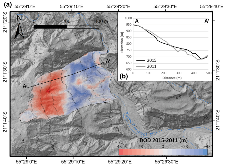
Fig. 7 1.1 \text{ Mm}^3 landslide triggered by the cyclone Bejisa in 2014 in Salazie. (a) DEMs of Difference (DOD) at 5 m resolution in the area affected by the landslide, surrounded by the dotted line; the red (erosion) and blue (accumulation) zones reveal major topographic changes between 2011 and 2015 (acquisition years of the DEMs). The black line A–A' marks the ends of the 2011 and 2015 topographic profiles presented in (b) showing clear mass transfer
