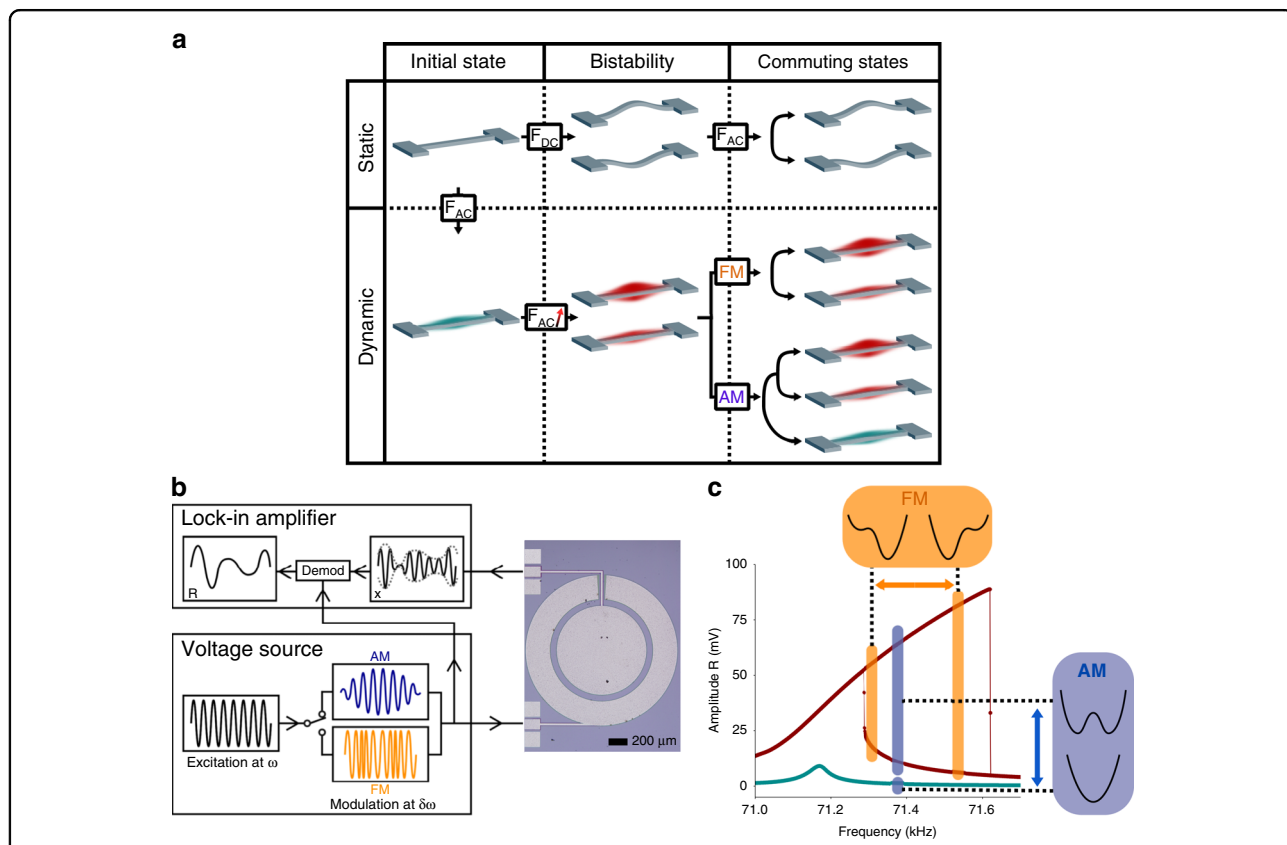
Fig. 1 Dynamic bistability for the generation of a chaotic regime in a nonlinear resonator. a Comparison between static and dynamic bistability for chaos generation in a nonlinear resonator, here represented by a doubly clamped beam. In the static case, a resonator reaches bistability through buckling by applying a static force F_{DC} while in the dynamic case, the alternative driving force F_{AC} is increased to enter the Duffing regime. By modulating the driving signal, the system evolves between the different states available, which results in a chaotic regime for an appropriate set of parameters. b Experimental setup. The MEMS (top view photography) is driven by a voltage source that provides the AM or FM configurations. The LIA demodulates the displacement x of the MEMS at the frequency of the source output to retrieve the amplitude R . c Amplitude response of the MEMS in the linear and Duffing regimes (dark cyan and dark red at 10 mV and 100 mV drive, respectively). The schematics qualitatively illustrate the evolution of the potentials involved for both the amplitude and frequency modulations (AM and FM) as a guide for the reader and are not meant for quantitative comparisons. In particular, the driving amplitudes and frequencies are far from the set of parameters used in the rest of the paper
