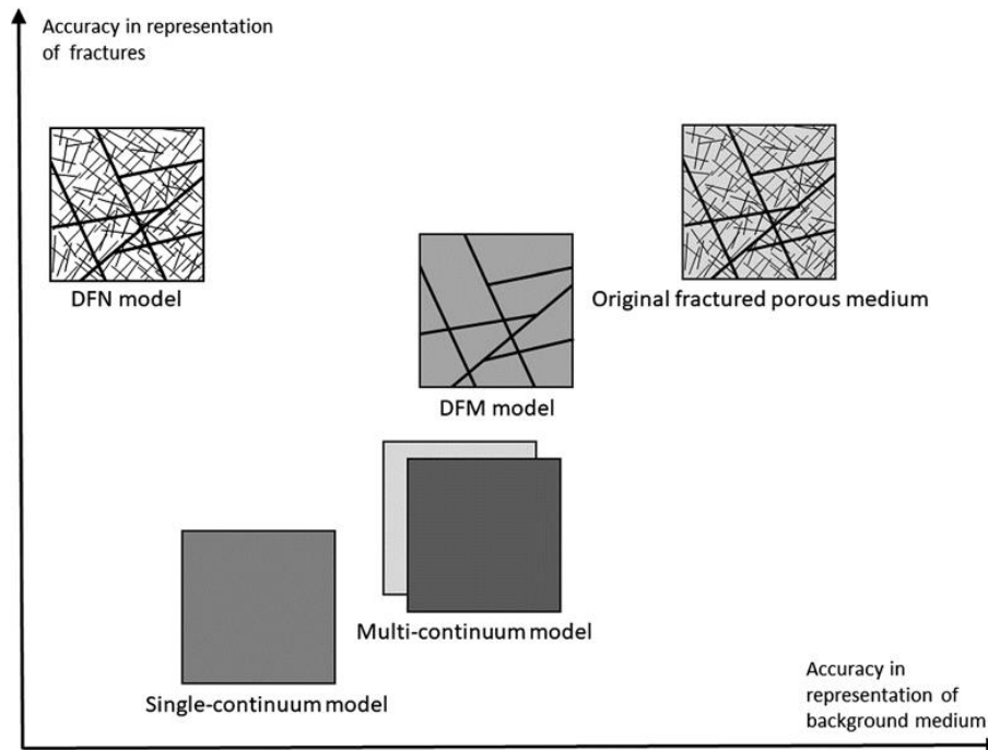
Figure 2: Conceptual approach for fractured porous media (Berre et al., 2019).
