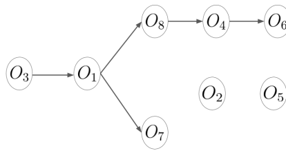
Fig. 1. Precedence graph
