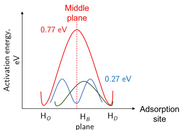
Fig. 3. Energy barrier corresponding to H_O , H_B , and H_D migration. It can be seen that a direct pathway from H_O to H_D costs 0.77 eV energy, however, a two-steps pathway is energetically cheaper.
