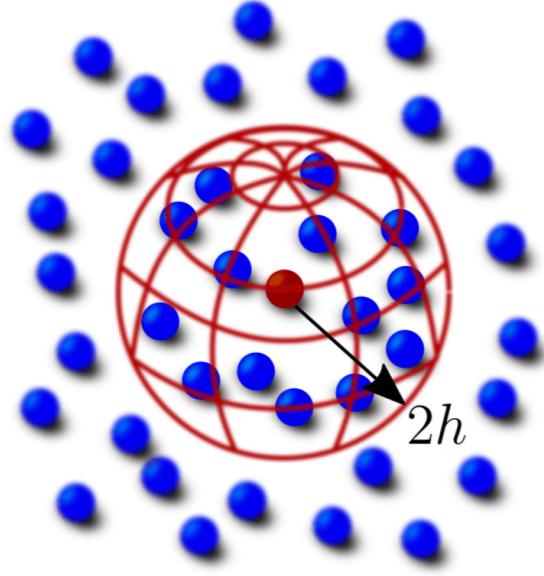
Figure 1: Particle approximation
