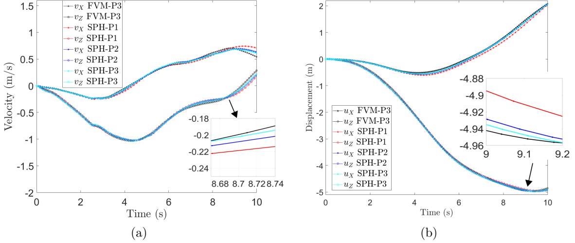
Figure 7: L-shaped block: time evolution of (a) components of velocity and (b) components of displacement at material point \mathbf{X} = [0, 10, 0]^T m. A comparison is carried out between the \{\mathbf{p}, \mathbf{F}, \mathbf{H}, J, E\} Upwind-VCFVM algorithm and the \{\mathbf{p}, \mathbf{F}, \mathbf{H}, J, E\} Upwind-SPH methodology. A polyconvex Mie-Grüneisen equation of state with properties Young’s modulus E = 50.05 KPa, density \rho_R = 1000 kg/m 3 , Poisson’s ratio \nu = 0.3 , thermal conductivity h = 10 Wm -1 K -1 , specific heat capacity C_v = 1 Jkg -1 K -1 , thermal expansion coefficient \alpha = 2.223 \times 10^{-4} K -1 , reference temperature \theta_R = 293.15 K and \alpha_{\text{CFL}} = 0.3 . P1, P2 and P3 represent 1900, 5400 and 17600 number of particles/nodes.
