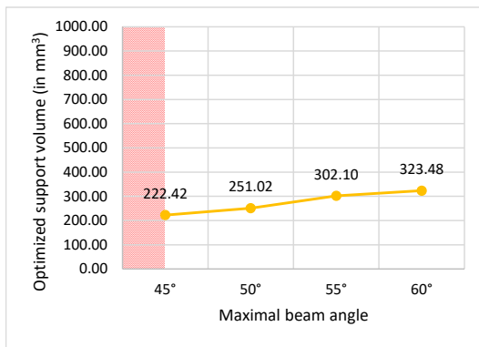
Figure 11: Volumes of optimized internal supports for the Stanford Bunny according to the initial lattice maximal beam angle \alpha_{max} . (unmanufacturable area in red)
