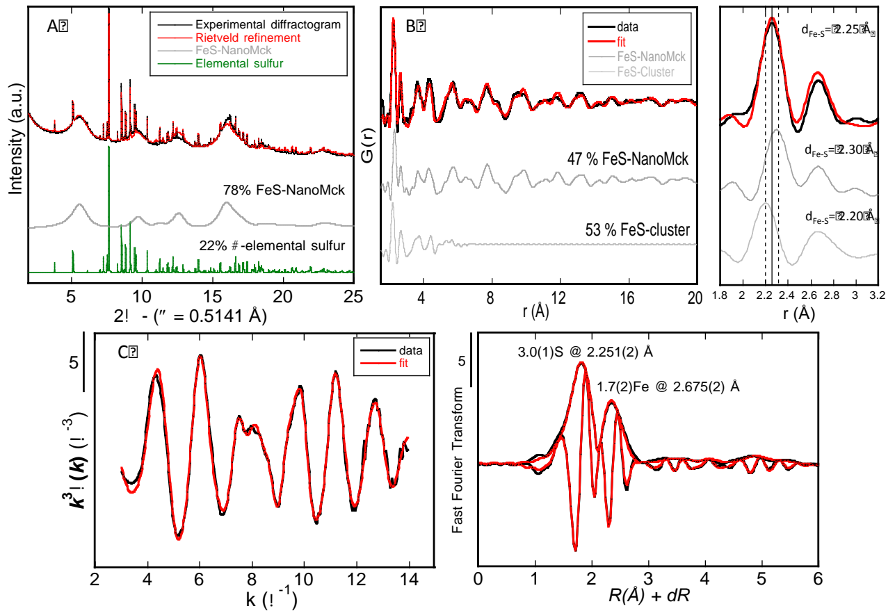
Figure 4. Detailed mineralogical analysis of the sample Fe-S 0.5h . Experimental and calculated curves are plotted in black and red colours, respectively. A. Rietveld refinement of the powder X-Ray diffraction pattern. The mineralogical phases observed are nanocrystalline mackinawite (78%) and \alpha -elemental sulfur (22%); refined crystallographic parameters are reported in Table 4. B. Pair Distribution Function (PDF) analysis. The best-fit solution is obtained from the refinement in real space of two FeS populations with different coherent size domains: FeS-NanoMck (47%) and FeS-cluster (53%). Refined parameters are reported in Table 4. C. Results of the shell-by-shell fitting procedure applied to the Fe K -edge k^3 -weighted EXAFS spectrum over the 3-14 k -range using phase-shift and amplitude functions simulated using the ab initio Feff8.1 code (Ikogou et al. , 2017). Fitting parameters are given in Table 4 and compared to the theoretical parameters of crystalline mackinawite (Lennie et al. , 1995). Fitting parameters of the shell-by-shell fitting procedure are listed in Table 5.
