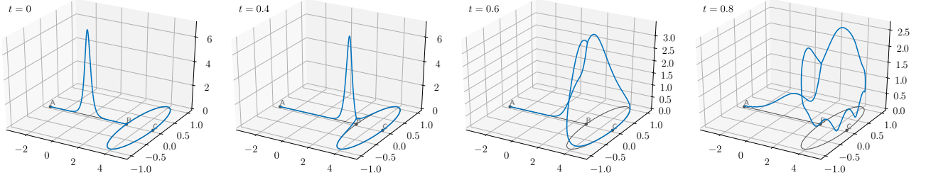
FIGURE 15. Simulation of (7) at times T = 0, 0.4, 0.6, 0.8 with the relaxation scheme.
