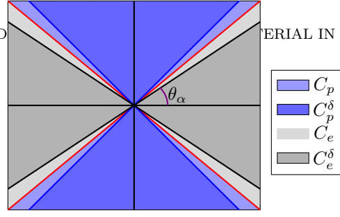
FIG. 2.1. The domains C_p^\delta , C_e^\delta , C_p , C_e , with \theta_\alpha = \text{atan } \alpha^{-1} .
