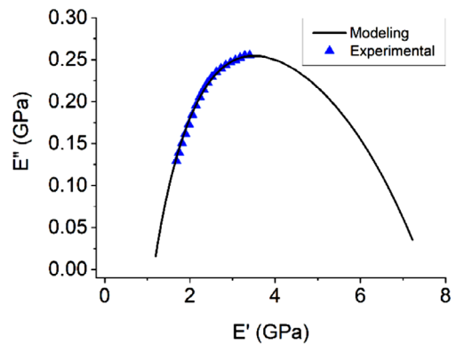
FIGURE 6 Cole-Cole plot of randomly-oriented low-density sheet molding compound composite [Color figure can be viewed at wileyonlinelibrary.com ]
