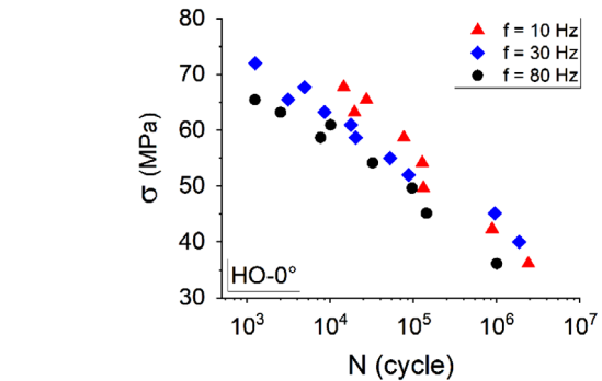
FIGURE 9 Wöhler curves at different frequencies in tension-tension tests for HO-0° samples. HO, highly-oriented [Color figure can be viewed at wileyonlinelibrary.com]
