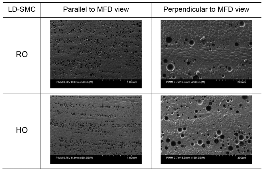
FIGURE 4 The microstructure of LD-SMC: Bundle of fibers and hollow glass spheres. HO, highly-oriented; LD-SMC, low-density sheet molding compound; MFD, mold flow direction; RO, randomly-oriented
