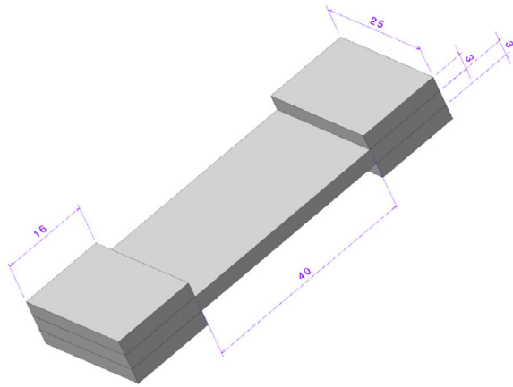
FIGURE 2 Specimen geometry (in mm) for damage analysis in fatigue [Color figure can be viewed at wileyonlinelibrary.com]
