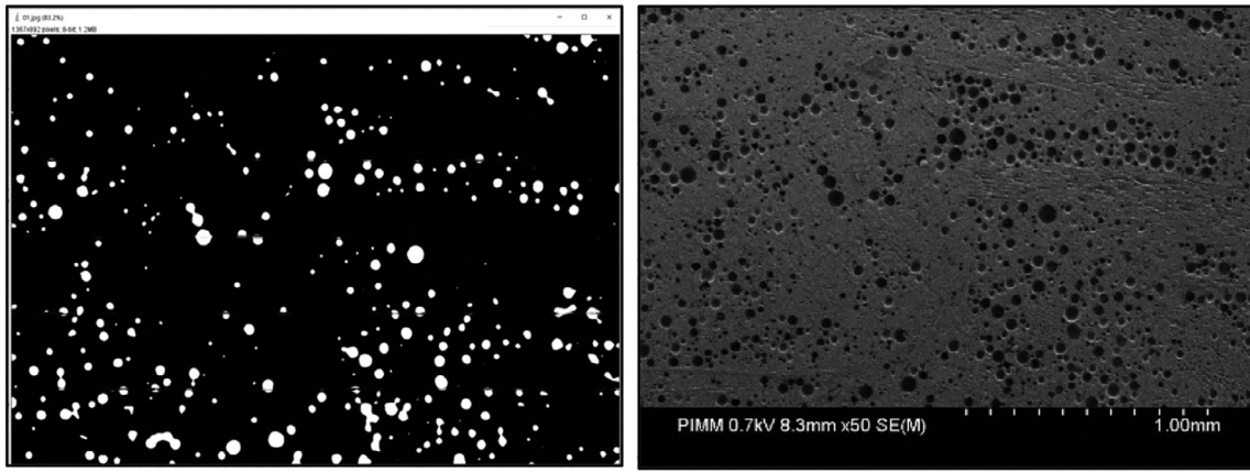
FIGURE 3 The microstructure of randomly-oriented low-density sheet molding compound: Homogeneous presence of hollow glass spheres
