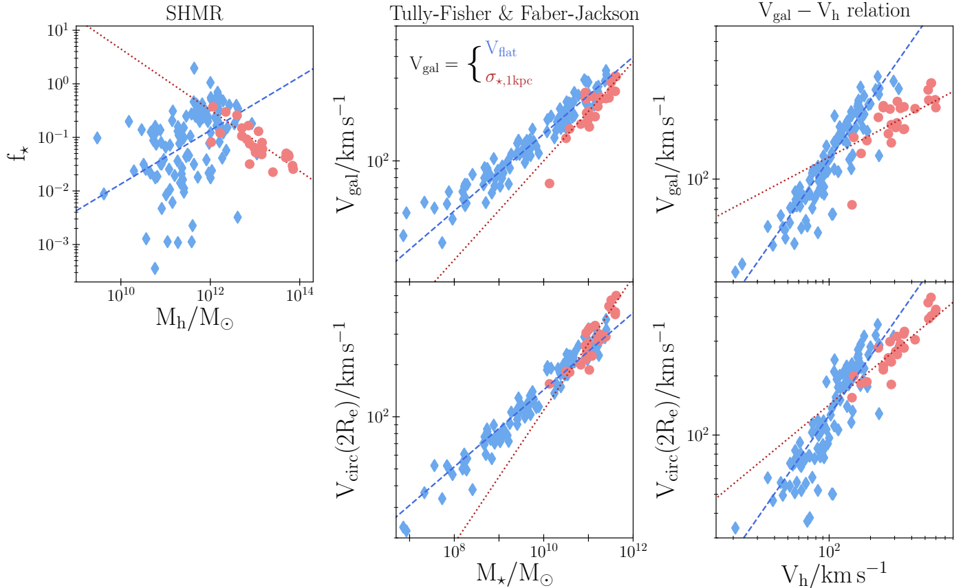
Fig. 10. SHMR ( f_* – M_h , left), stellar mass-velocity scaling law ( M_* – V_{\text{gal}} , middle), and the relation between galaxy velocity and halo velocity ( V_{\text{gal}}-V_h , right) for the population of late types (blue) and massive early types (red). Top-middle and top-right panels: the characteristic velocity of galaxies V_{\text{gal}} is the velocity along the flat parts of HI rotation curves for late types ( V_{\text{flat}} , Lelli et al. 2016b) and the velocity dispersion of stars within 1 kpc for early types ( \sigma_{*,1\text{kpc}} , Brodie et al. 2014). Bottom-middle and bottom-right panels: we substitute the observed V_{\text{gal}} with the circular velocity evaluated at the same radius ( 2R_e ) for both galaxy types. In all panels, we show power-law fits to the data of late types (blue dashed lines) and early types (red dotted lines).
