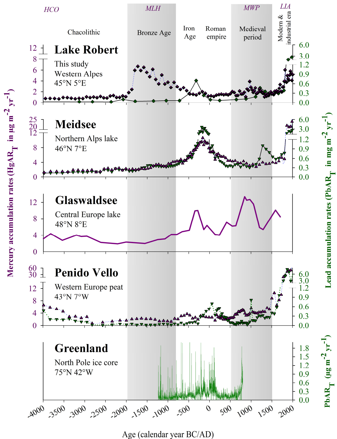
Fig. 7: Pb and Hg \text{AR}_T in lake Robert record compared to selected European records: lake Meidsee (Thevenon et al., 2011), Lake Glaswaldsee (Schütze et al., 2018), Penido Vello (Martinez-Cortizas et al., 1999, 1997) and to Greenland Ice record (McConnell et al., 2018)
