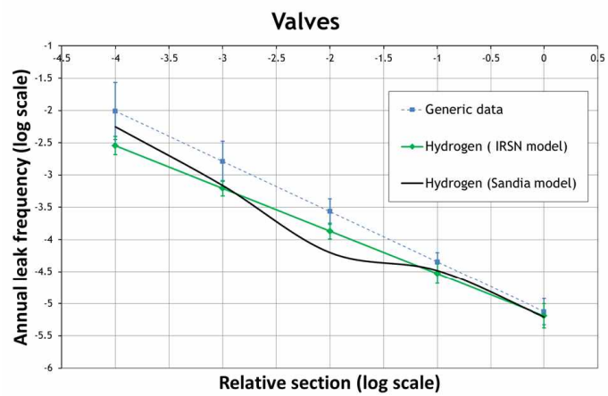
Fig. 5. Results obtained by IRSN for the second step of the sequential bayesian modeling seals; compressors; valves
