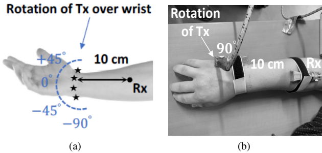
Fig. 2. (a) The proposed configuration of Tx-Rx for wrist to arm channel gain measurements in the 55-65 GHz range. (b) VV-configuration of two horn antennas on an arm with Tx rotated 90° relative to Rx at a separation distance of 10 cm.
