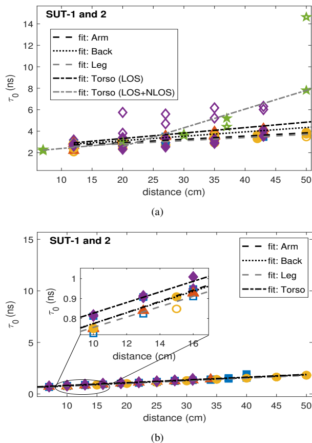
Fig. 6. Mean excess delay ( \tau_0 ) measured (markers) for HH antennas on both subjects as a function of distance between Tx-Rx. (a) 900-MHz (b) 60 GHz. Measurements on SUT-1 and SUT-2 are indicated with empty and filled markers, respectively. Square: arm, Triangle: back, Circle: leg, Diamond: torso (LOS) and Pentagon: torso (LOS+NLOS).
