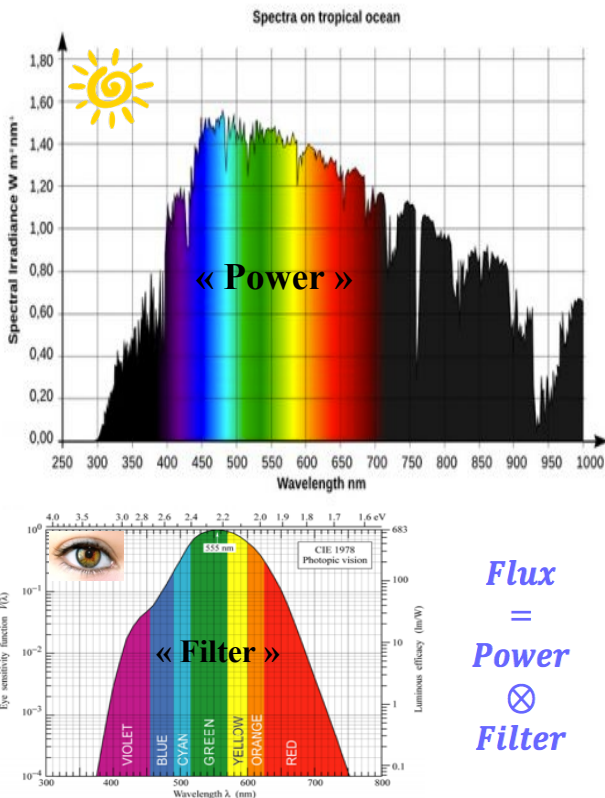
Fig. 5. Full sun spectrum at sea level, Human eye perception [9] and Lumen definition
