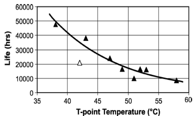
Fig. 4. Lifetime vs temperature for White Light LED [8].
