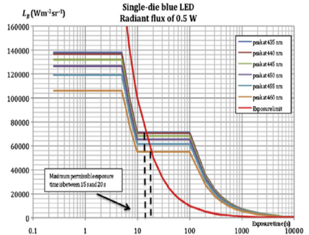
Fig. 9. Luminance VS exposure time to light / maximum permissible exposure without damage.
