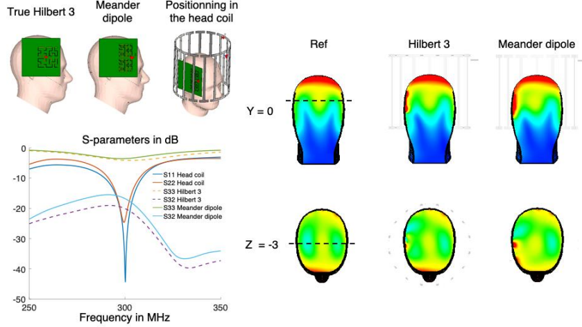
Fig. 1. Design and study of original Hilbert fractal and meander dipole. Top left, structures' design and position with respect to the head and the coil. Bottom left, S-parameters showing the coupling between the structures and the head coil. Right side, Amplitude of B_1^+ field on Y direction at the center of the phantom and Z direction at -3 cm below the center. The dash lines show the position where the slices were obtained, color scale from 0 to 0.5 \mu\text{T} .
