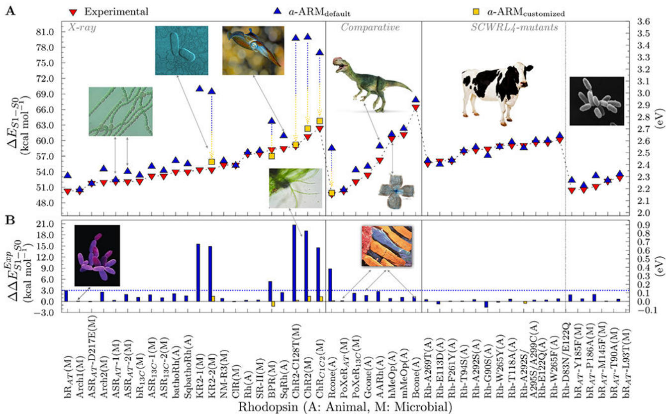
Fig. 20. Benchmarking of a -ARM. (A) Computed excitation energies E_{S1-S0} in both \text{kcal mol}^{-1} (left axis) and eV (right axis) for various rhodopsins. The employed protein structures were obtained from X-ray crystallography (left panel) or through comparative modeling (center panel). Two sets of variants for bovine rhodopsin (Rh) and bacteriorhodopsin (bR) are also reported (right panel). The computed data were obtained using the a -ARM default (blue up-turned triangles) and a -ARM customized (gold squares). Experimental data, as energy difference corresponding to the wavelength of the absorption maxima, are also reported (red down-turned triangles). (B) Differences between computed and experimental excitation energies E^{\text{Exp}}_{S1-S0} in both \text{kcal mol}^{-1} (left axis) and eV (right axis).
