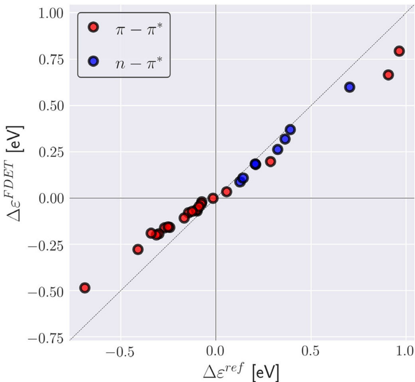
Fig. 15. Environment-induced shifts of the lowest vertical excitation energy for organic chromophores in hydrogen-bonded environments (XH-27 dataset from Ref. (144)). Reference shifts ( \epsilon^{ref} ) are taken Ref. (144) (excitation energy shifts obtained from ADC(2) calculations for the whole clusters). FDET shifts ( \epsilon^{FDET} ) are obtained from embedded ADC (2) calculations as described in Ref. (144) except the reduction of the number of centers in the basis sets used for \Psi_A and \rho_B (monomer expansion is used here).
