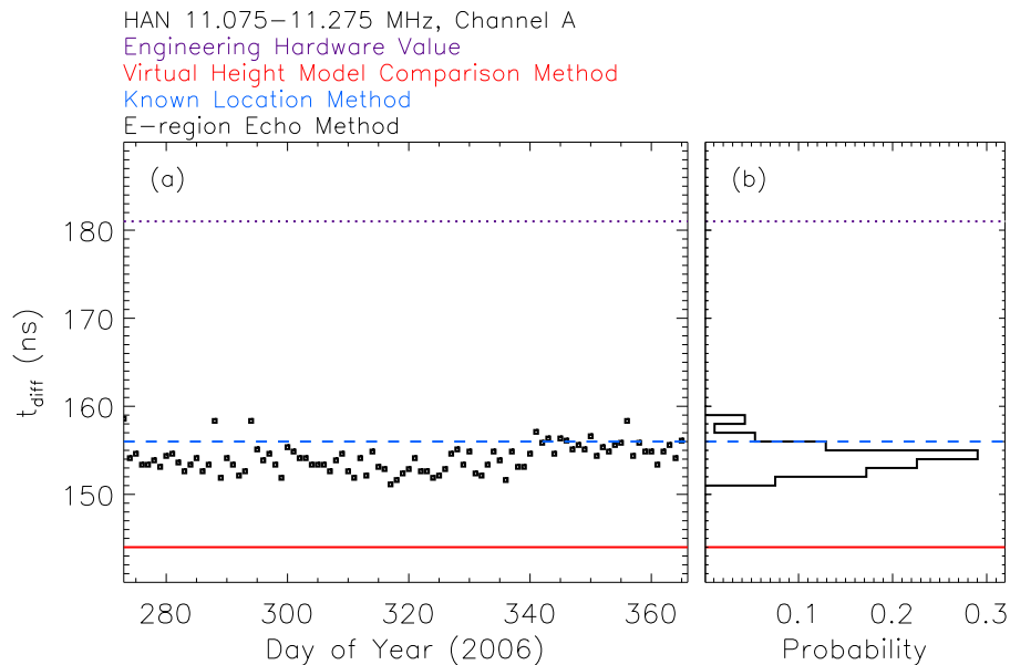
Fig. 4. Comparison between the results of different t_{diff} estimation methods for the HAN radar for the last 3 months of 2006. The estimates have been determined for the Channel A 11.075–11.275 MHz frequency band, with a 2\pi integer ambiguity added (where necessary) to obtain the t_{diff} estimate closest to the hardware value of 181 ns. (a) The black symbols represent the estimates from the E-region method. The blue dashed line and the solid red line represent the estimates from the Known Location and VHM comparison methods, respectively, over the interval that they were valid. The purple and white horizontal dotted line at 181 ns represents the hardware value. (b) The t_{diff} estimate histogram for the E-region method for the same interval. The blue and red lines represent the t_{diff} estimates from the Known Location and VHM comparison methods, respectively, which were constant over this evaluation period. The purple and white horizontal dotted line again represents the hardware value of 181 ns. (For interpretation of the references to colour in this figure legend, the reader is referred to the web version of this article.)
