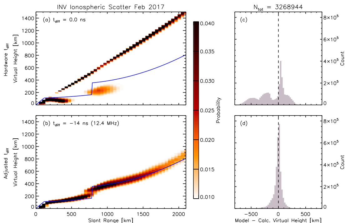
Fig. 1. Comparison of virtual height distributions when using the hardware t_{diff} (0.0 ns) and the t_{diff} found by adjusting the \frac{1}{2} hop ionospheric backscatter to match the Chisham VHM (-14 ns at 12.4 MHz). Panels (a) and (b) show two-dimensional histograms of the slant range and virtual height distribution of the INV data from February 2017 for ranges 0–2100 km, with the VHM overlaid in blue. Panels (c) and (d) show histograms of the difference between the modelled and measured virtual heights at these same ranges. (For interpretation of the references to colour in this figure legend, the reader is referred to the web version of this article.)
