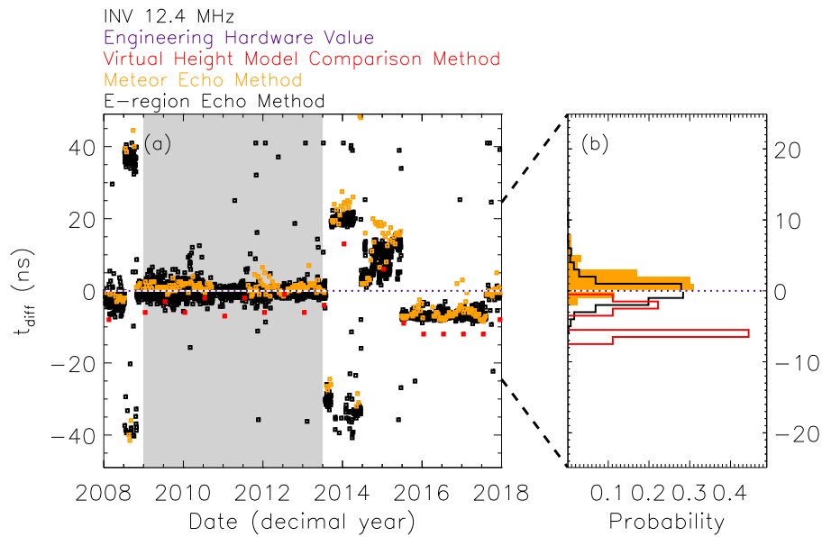
Fig. 3. Comparison between the results of different t_{\text{diff}} estimation methods for the INV radar for the interval 2008 to 2017 inclusive. The estimates have been determined for a frequency band centred around 12.4 MHz, with a 2\pi integer ambiguity added (where necessary) to obtain the t_{\text{diff}} estimate closest to the hardware value of zero. (a) The black, orange, and red symbols represent the estimates from the E-region, meteor scatter, and VHM comparison methods, respectively. The purple and white horizontal dotted line at 0 ns represents the hardware value. (b) t_{\text{diff}} estimate histograms for the interval January 2009 to June 2013 inclusive. This interval is marked by the grey region in panel (a). The black, orange, and red histograms represent the t_{\text{diff}} estimate distributions from the E-region, meteor scatter, and VHM comparison methods, respectively. The purple and white horizontal dotted line again represents the hardware value of 0 ns. (For interpretation of the references to colour in this figure legend, the reader is referred to the web version of this article.)
