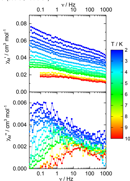
Figure 3. Frequency dependences of both in-phase, \chi_M' , and out-of-phase, \chi_M'' , components of the ac susceptibility for 5 at zero external dc field between 2 and 10 K.
