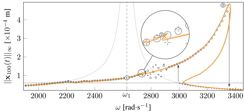
Figure 9 – NRFC obtained with the TI reference strategy (upward (o) and downward (+) frequency sweeps), by R-HBM (—) and RL-HBM (—). Linear FRF (—) and contact threshold (—).
