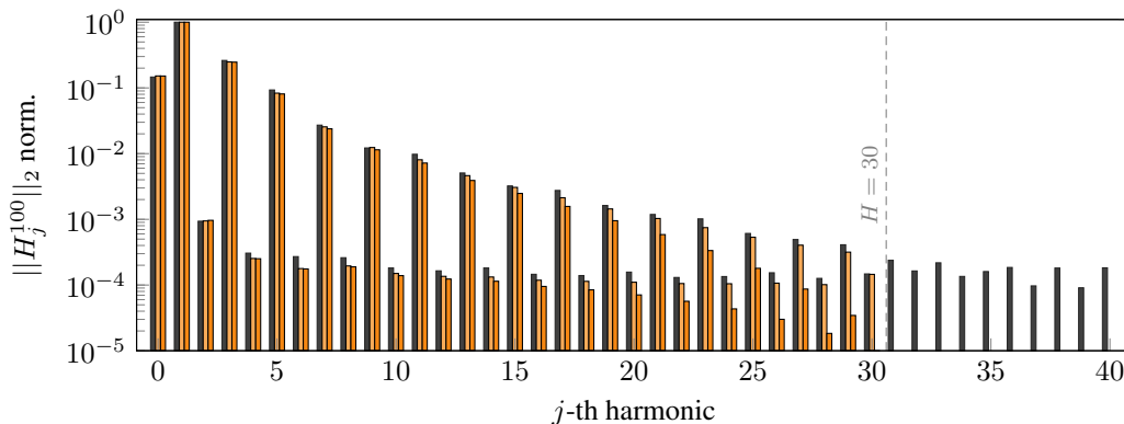
Figure 10 – Frequency spectra of solutions obtained at \omega_1 = 2628 \text{ rad}\cdot\text{s}^{-1} ① with the TI reference strategy (■), R-HBM (■) and RL-HBM (■).
