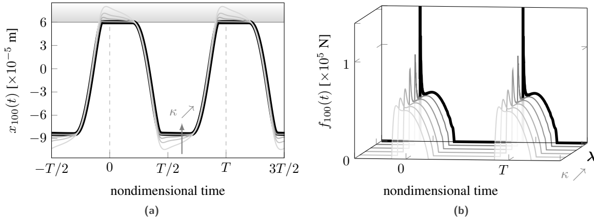
Figure 7 – Steady states obtained with the TI reference strategy for \omega_1 = 2628 \text{ rad}\cdot\text{s}^{-1} , with the penalty method for \kappa = \{3.3 \cdot 10^9, 6.3 \cdot 10^9, 1.3 \cdot 10^{10}, 6.3 \cdot 10^{10}, 1.3 \cdot 10^{11}\} \text{ N}\cdot\text{m}^{-1} (—) and Lagrange multipliers \lambda (—): (a) displacements and (b) normal contact forces.
