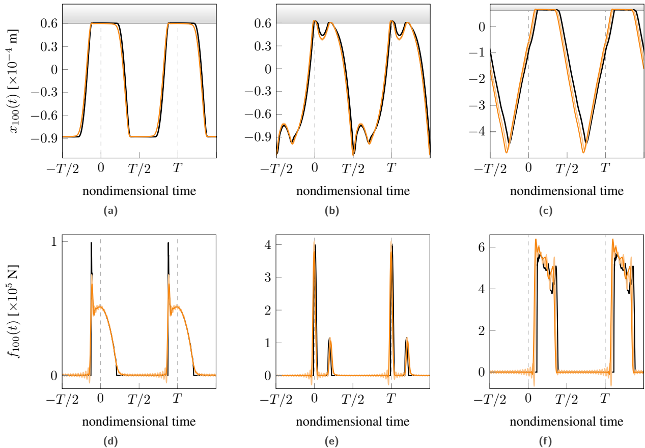
Figure 12 – Solutions obtained with the TI reference strategy (—), R-HBM (—) and RL-HBM (—). Displacements and contact forces for areas: (a) (d) ①, (b) (e) ②, and (c) (f) ③.
