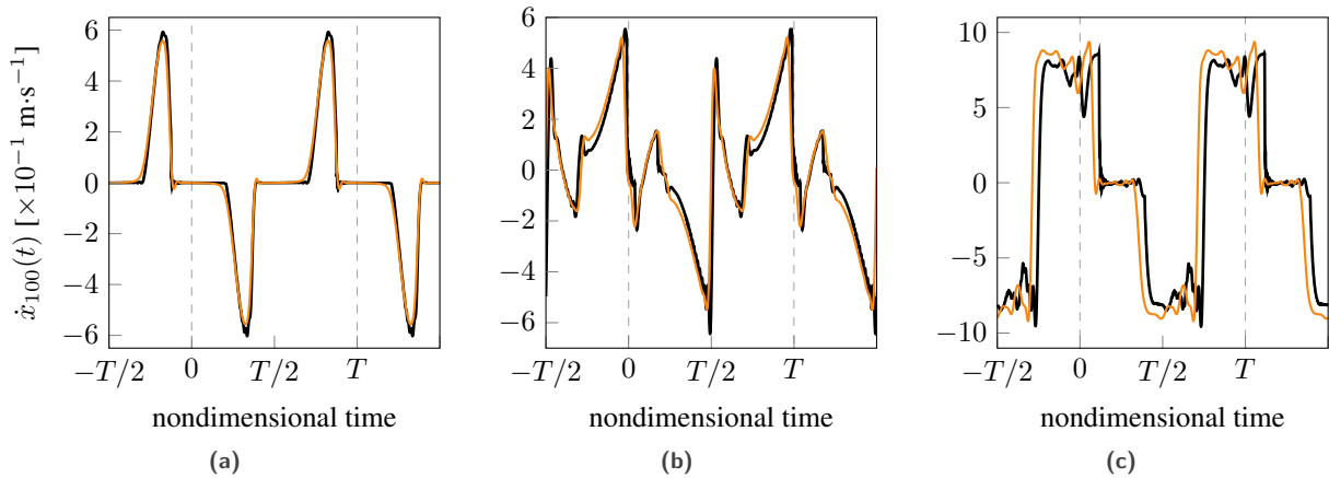
Figure 14 – Velocities obtained by RL-HBM (—) and TI reference strategy (—) for areas: (a) ①, (b) ②, and (c) ③.
