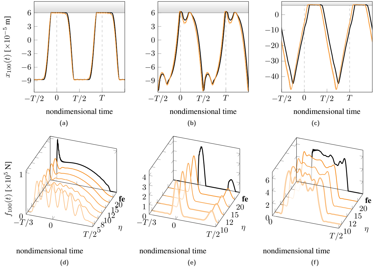
Figure 13 – Solutions obtained by RL-HBM (—) for various reduction parameter \eta and TI reference strategy (—) on full finite element model (fe). Displacements and contact forces for areas: (a) (d) ①, (b) (e) ②, and (c) (f) ③.
