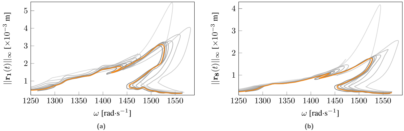
Figure 17 – NFRC computed with RL-HBM ( N = 1024 ) for H = \{5 (—), 10 (—), 15 (—), 20 (—), 25 (—), 30 (—), 35 (—), 40 (—), 80 (—)} at (a) LE and (b) TE.
