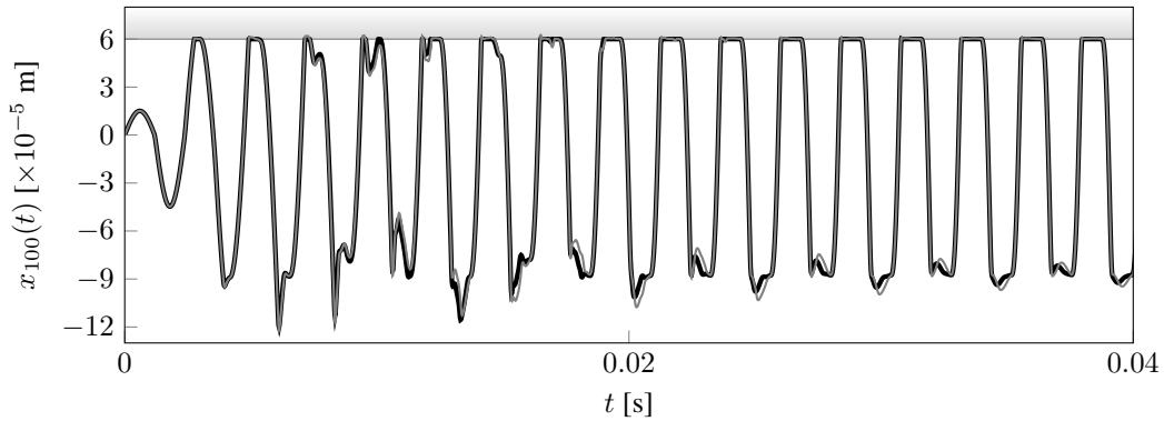
Figure 8 – Transient time responses obtained with Lagrange multipliers (—) and penalty method for \kappa = 1.3 \cdot 10^{11} \text{ N}\cdot\text{m}^{-1} (---).
