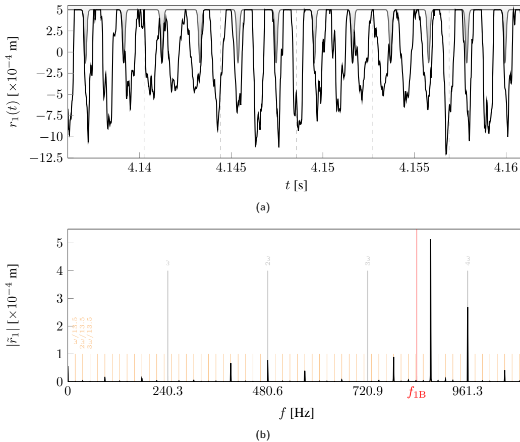
Figure 25 – 13.5- T -periodic solution obtained with TI at \omega = 1510 \text{ rad}\cdot\text{s}^{-1} : (a) displacements over revolutions 995 to 1000 and (b) FFT frequency spectrum.
