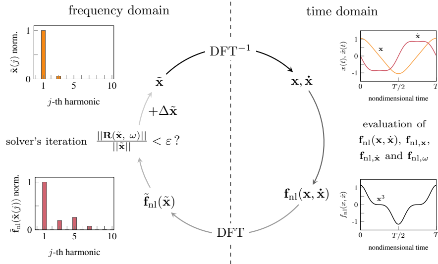
Figure 3 – Illustration of the alternating frequency/time scheme.
