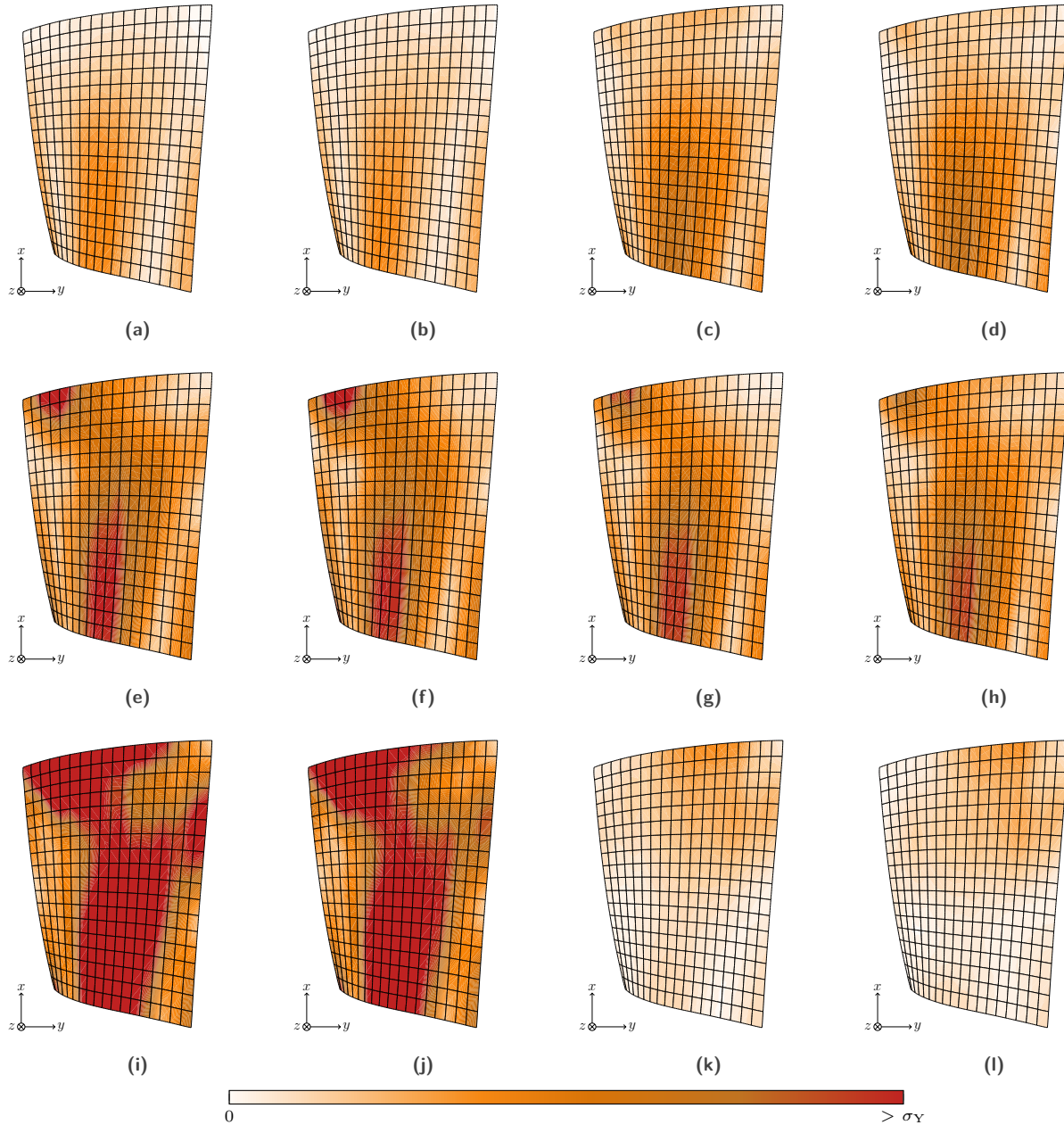
Figure 24 – Comparison between resulting von Mises stress obtained with RL-HBM and TI at corresponding HBM maximal displacement instant. RL-HBM for areas: (a) ① \sigma_{\max} = 0.429 \sigma_Y , (c) ② \sigma_{\max} = 0.777 \sigma_Y , (e) ③ \sigma_{\max} = 1.012 \sigma_Y , (g) ④ \sigma_{\max} = 0.941 \sigma_Y , (i) ⑤ \sigma_{\max} = 1.674 \sigma_Y and (k) ⑥ \sigma_{\max} = 0.406 \sigma_Y . TI for areas: (b) ① \sigma_{\max} = 0.404 \sigma_Y , (d) ② \sigma_{\max} = 0.767 \sigma_Y , (f) ③ \sigma_{\max} = 0.993 \sigma_Y , (h) ④ \sigma_{\max} = 0.91 \sigma_Y , (j) ⑤ \sigma_{\max} = 1.587 \sigma_Y and (l) ⑥ \sigma_{\max} = 0.425 \sigma_Y .
