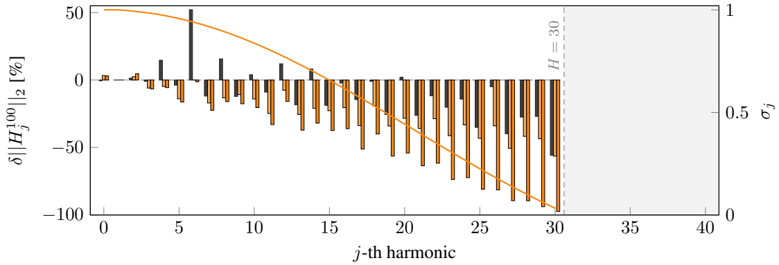
Figure 11 – Differences between the frequency spectra of the solutions obtained at \omega_1 = 2628 \text{ rad}\cdot\text{s}^{-1} ① by the TI reference strategy (■), R-HBM (□) and RL-HBM (▣) with respect to the standard HBM. Lanczos filter profile (—).
