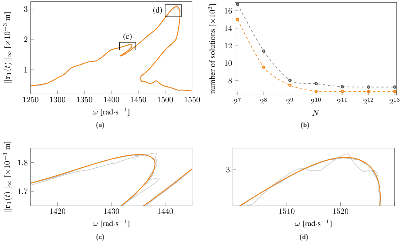
Figure 18 – NFRC computed with RL-HBM ( H = 40 ) for N = \{2^7 = 128 (—), 256 (—), 512 (—), 1024 (—), 2048 (—), 2^{13} = 4096 (—)} (a) full NFRC, (b) number of the NFRC solutions points with (—○—) and without (—●—) Lanczos filtering, (c) zoom over the turning area and (d) nonlinear resonance.
