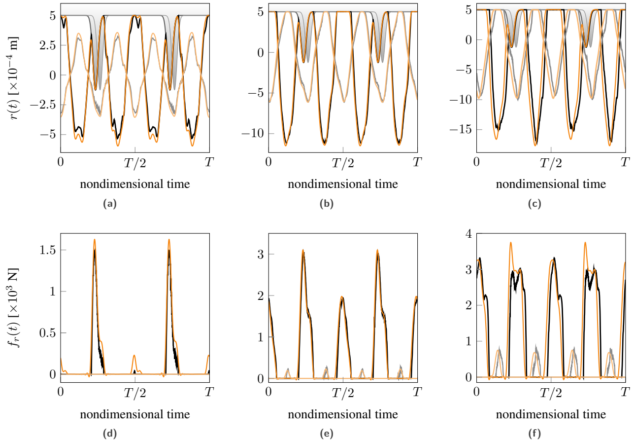
Figure 21 – Comparison between radial displacements and contact forces obtained by RL-HBM and TI at LE and TE for areas: (a) (d) ①, (b) (e) ②, and (c) (f) ③. Legends: TI LE (—), TE (—), RL-HBM LE (—) and TE (—).
