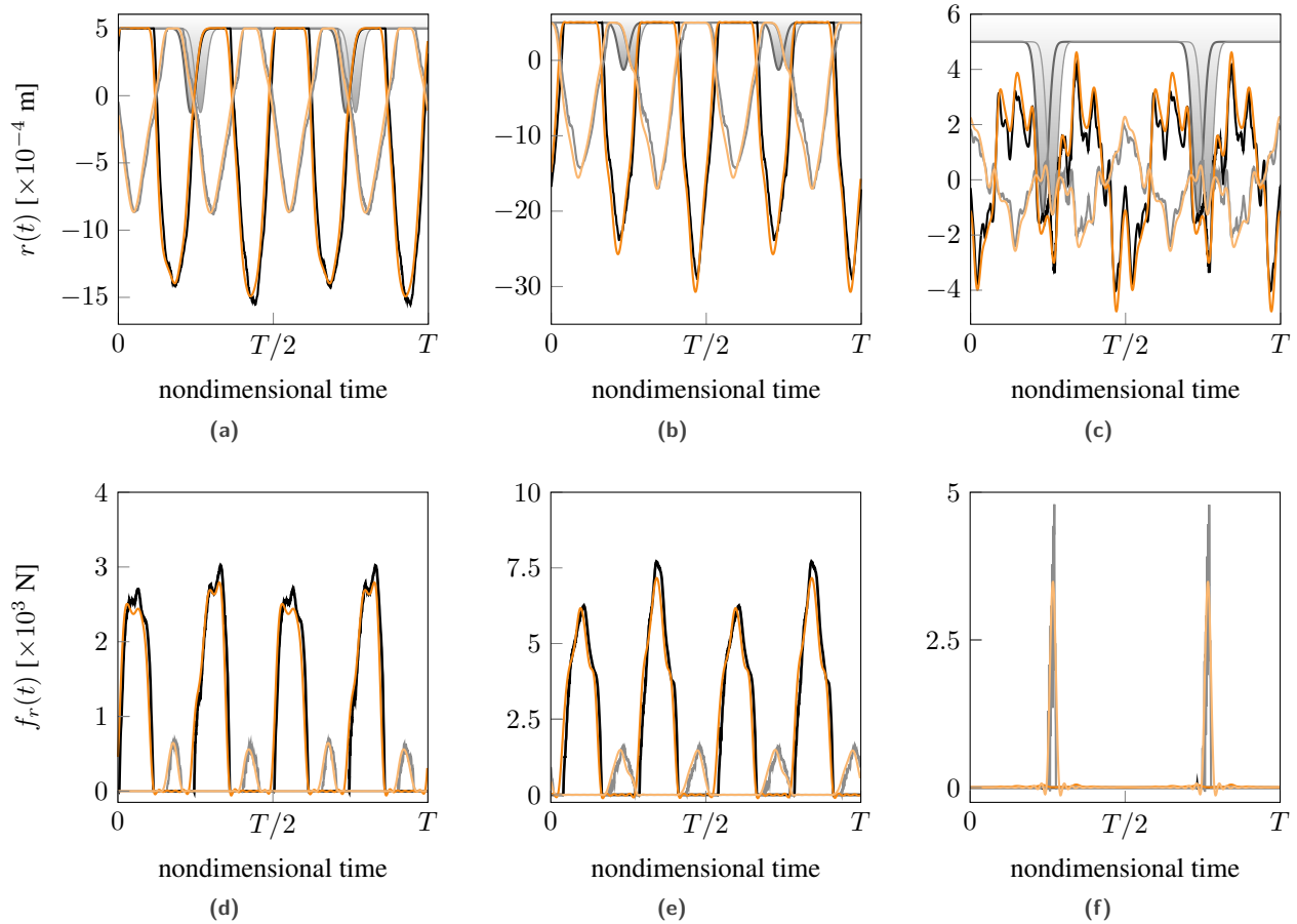
Figure 22 – Comparison between radial displacements and contact forces obtained by RL-HBM and TI at LE and TE for areas: (a) (d) ④, (b) (e) ⑤, and (c) (f) ⑥. Legends: TI LE (—), TE (—), RL-HBM LE (—) and TE (—).
