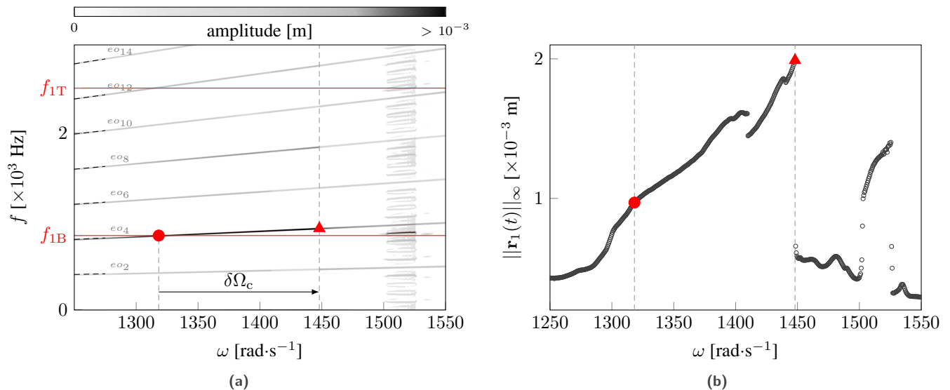
Figure 1 – Numerical results for a test case of blade-tip/casing contact: (a) interaction map and (b) nonlinear frequency response curve.
