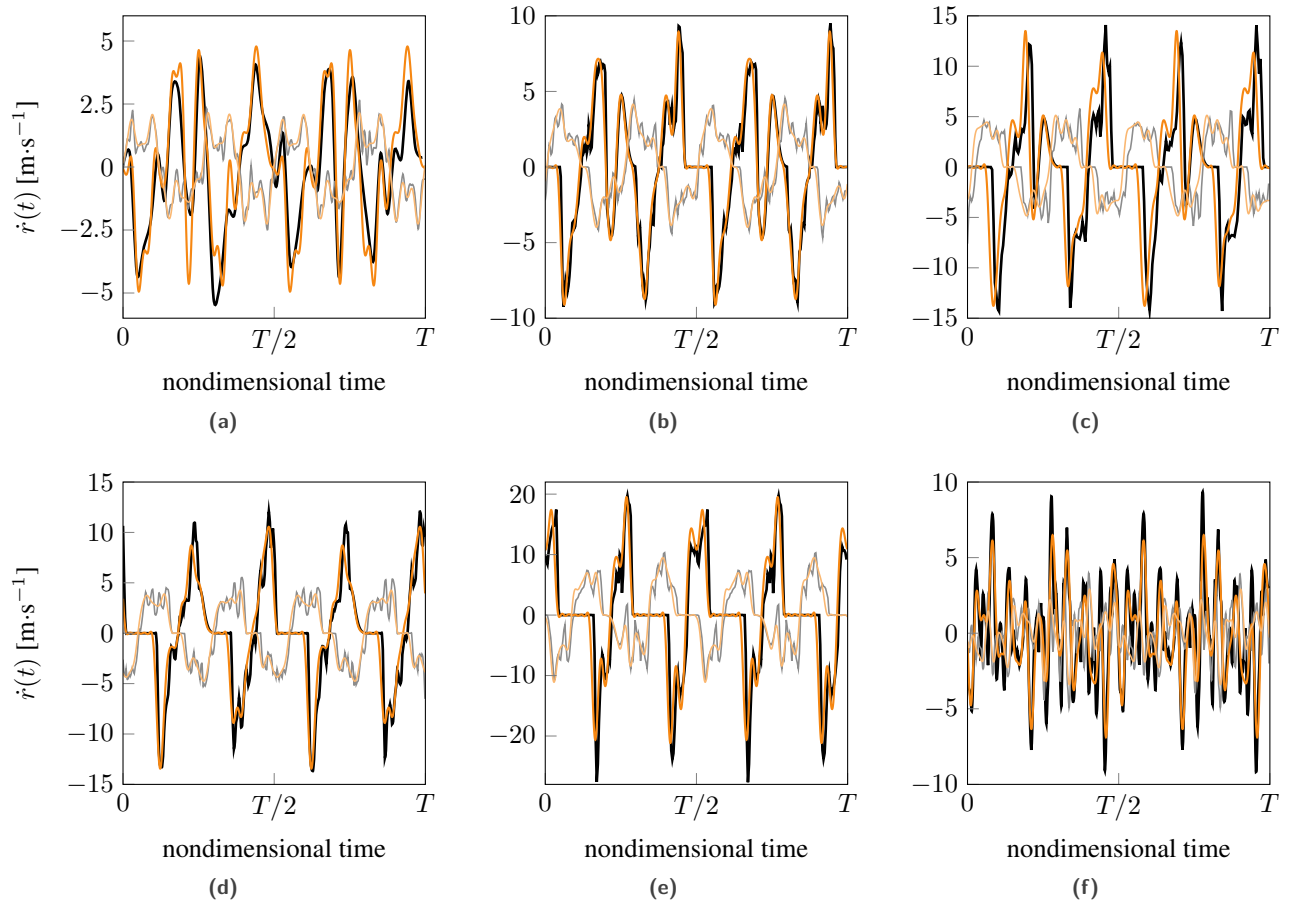
Figure 23 – Comparison between radial velocities obtained by RL-HBM and TI at LE and TE for areas: (a) ①, (b) ②, (c) ③, (d) ④, (e) ⑤ and (f) ⑥. Legends: TI LE (—), TE (—), RL-HBM LE (—) and TE (—).
