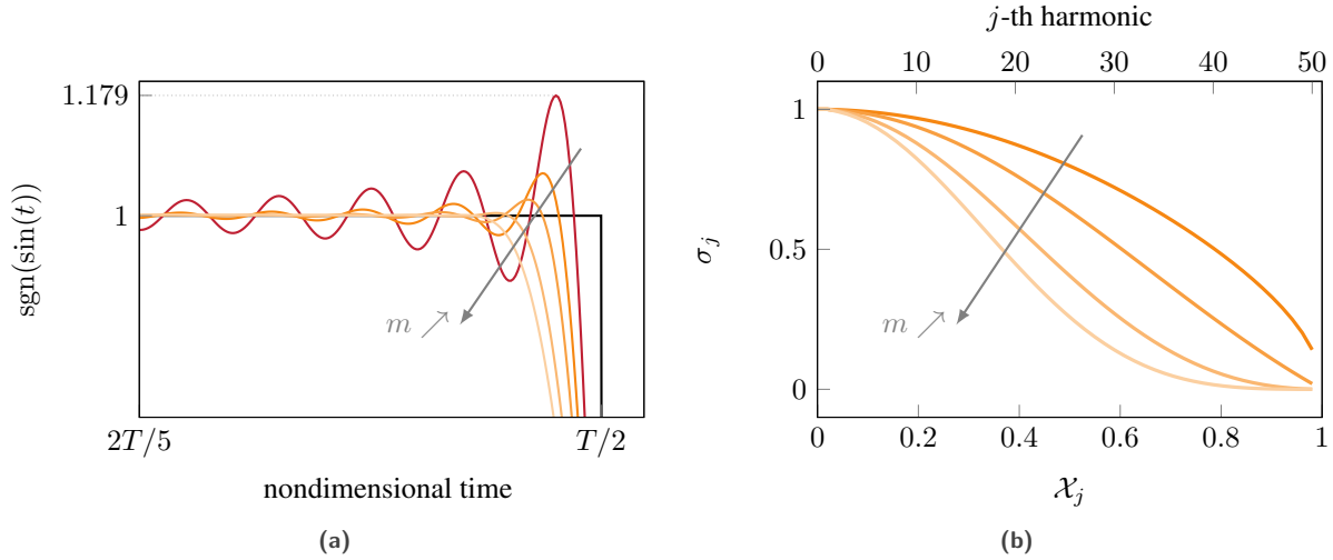
Figure 5 – Illustration of the Lanczos filtering technique: (a) Gibbs phenomenon for the approximation of a T -periodic square wave (—) by a Fourier series truncated at H = 50 (—) and with Lanczos filter for different values of m , and (b) Lanczos factors obtained with different m . Legends: m = 0.5 (—), m = 1 (—), m = 2 (—) and m = 3 (—).
