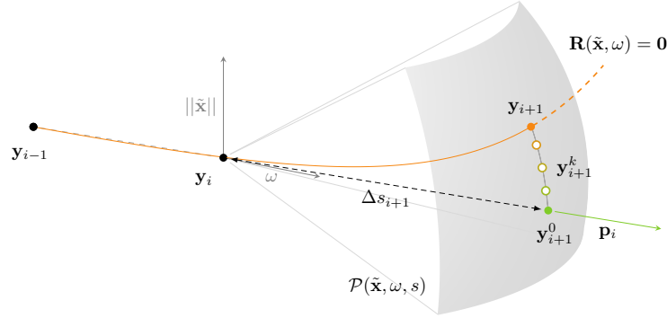
Figure 2 – Principle of the arc-length continuation technique: known solutions (●), prediction (●) and new solution (●).
