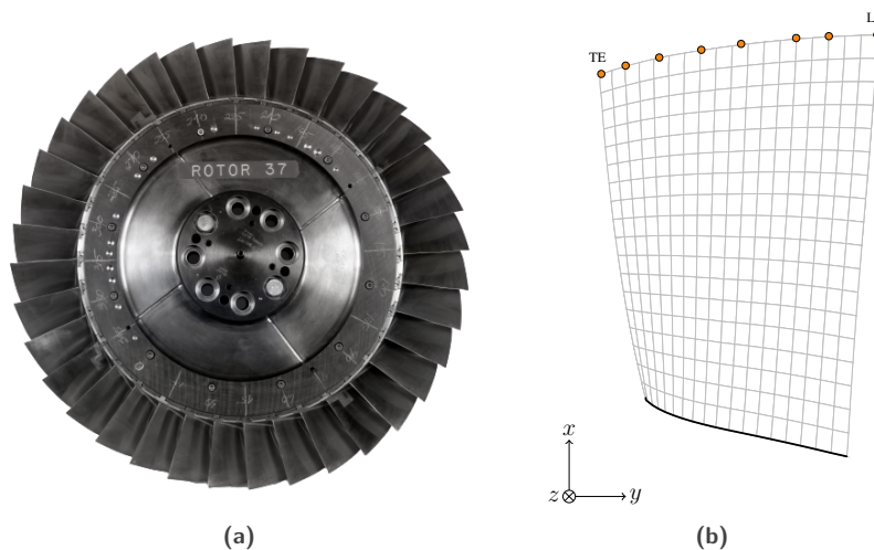
Figure 15 – NASA rotor 37: (a) full stage as shown in [49] and (b) finite element mesh of one blade.
