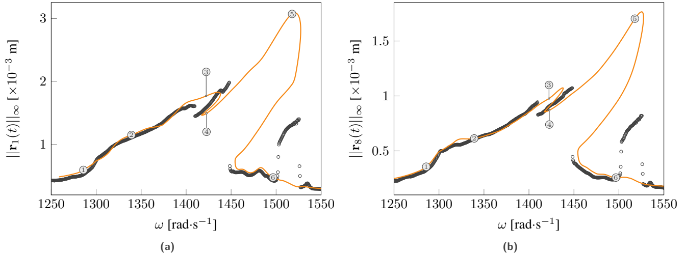
Figure 19 – NFRC of radial displacements obtained with TI (○) and RL-HBM (—) at (a) LE and (b) TE.
