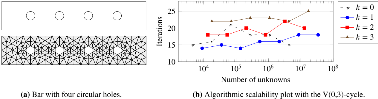
FIGURE 10 2D complex geometry and associated algorithmic scalability plot for the multigrid solver. The coarse meshes are built using the agglomeration coarsening strategy with face collapsing. The L^2 -orthogonal projection is computed exactly.
