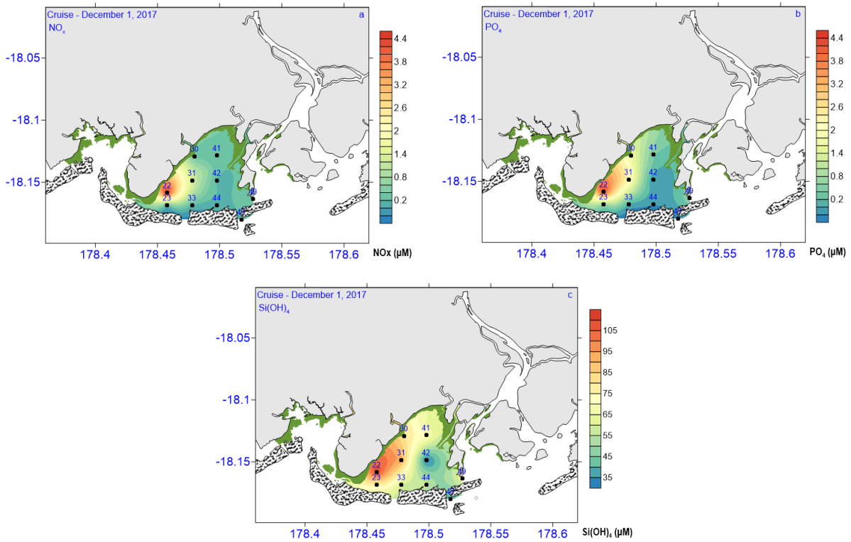
Figure 5. Color maps for biogeochemical variables (a) \text{NO}_x ; (b) \text{PO}_4 and (c) \text{Si(OH)}_4 .
