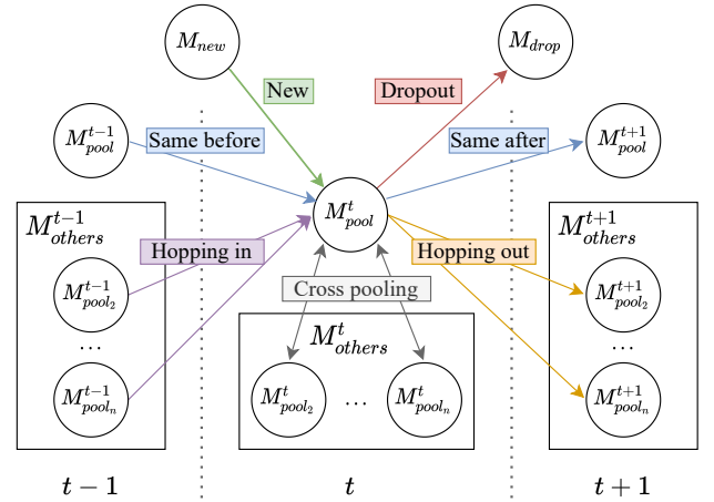
Fig. 3. The miners' migration flow model of pool at time interval t . t-1 ( t+1 ) is the time interval before (resp. after) t . M_{new} ( M_{drop} ) is the list of miners not in any pool at t-1 (resp. is not found in any mining pool at t+1 ). The union of the list of miners from other pools is M_{others} .
