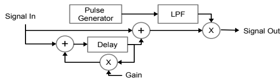
Figure 9. Block diagram of delayed-windowed voice processing
