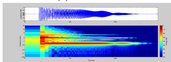
Figure 7. Waveform and Spectrogram of one Singing Bowl strike
