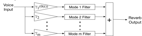
Figure 8. Block Diagram of Modal Reverberator Architecture
