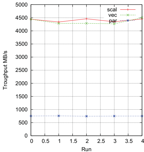
Figure 8. Stability of measures (copy1 on macro, icc version)
