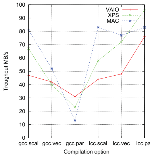
Figure 9. Freeverb.dsp benchmark
