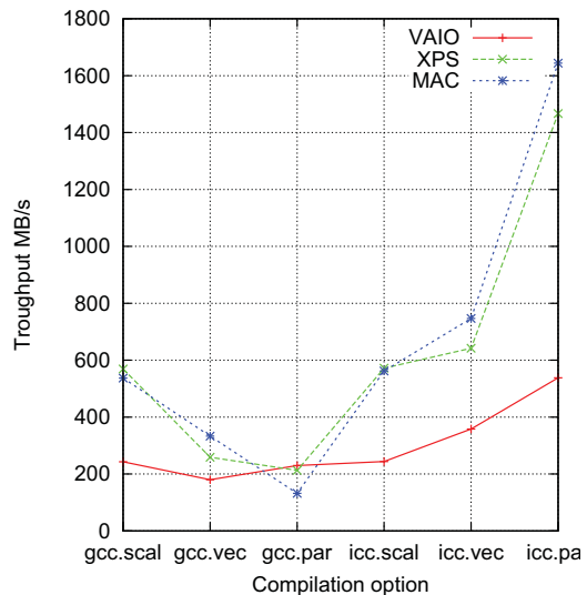
Figure 14. rms8.dsp benchmark
