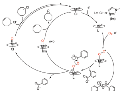
Scheme 1 Activation of O_2 catalyzed by Mn(TPP)Cl in CH_2Cl_2 , in the presence of benzoic anhydride, and 1-MeIm or Cl^- leading to oxygenation or chlorination of cyclooctene, respectively.
