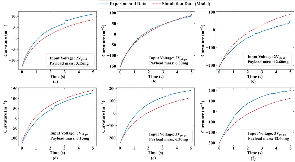
Fig. 7. Concurrence of experimental measurements with simulation results (model). Input voltage amplitudes— Up: 2V_{pk-pk} , with payload masses (a) 3.15 mg, (b) 6.30 mg, (c) 12.60 mg; Down: 3V_{pk-pk} , with payload masses (d) 3.15 mg, (e) 6.30 mg, and (f) 12.6 mg.
