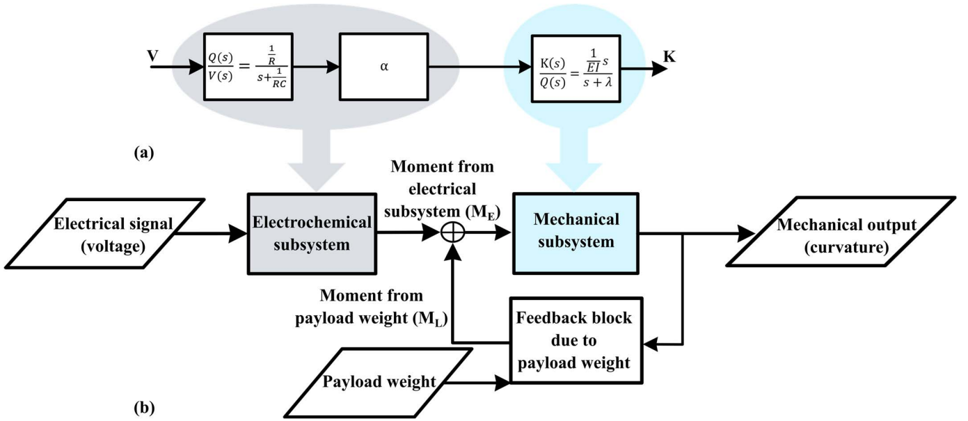
Fig. 2. Block diagram of the ionic actuator (a) Unloaded: subsystems with their relative transfer functions (b) Loaded: payload effect modeled as a feedback block.
