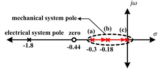
Fig. 6. System stability analysis: location of the actuator poles and zero. Mechanical subsystem pole for (a) an unloaded actuator, (b) a payload mass = 12.6 mg, and (c) marginal stability, calculated with a payload mass = 20 mg.
