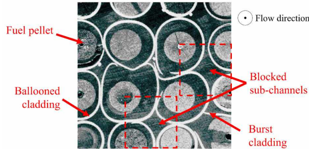
Figure 1: Clad ballooning and appearance of blocked sub-channels after an in-pile LOCA experiment (adapted from [1]).
