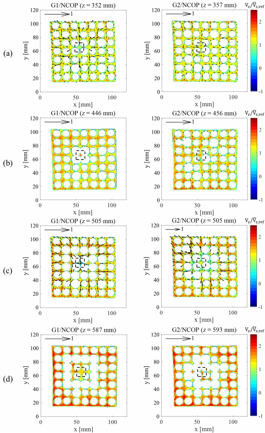
Figure 19: Velocity fields for different bundles comparing the blockage coplanarity effect - Part I. The sub-channel highlighted by the black box in each bundle was used to trace the profiles in Fig. 21.
