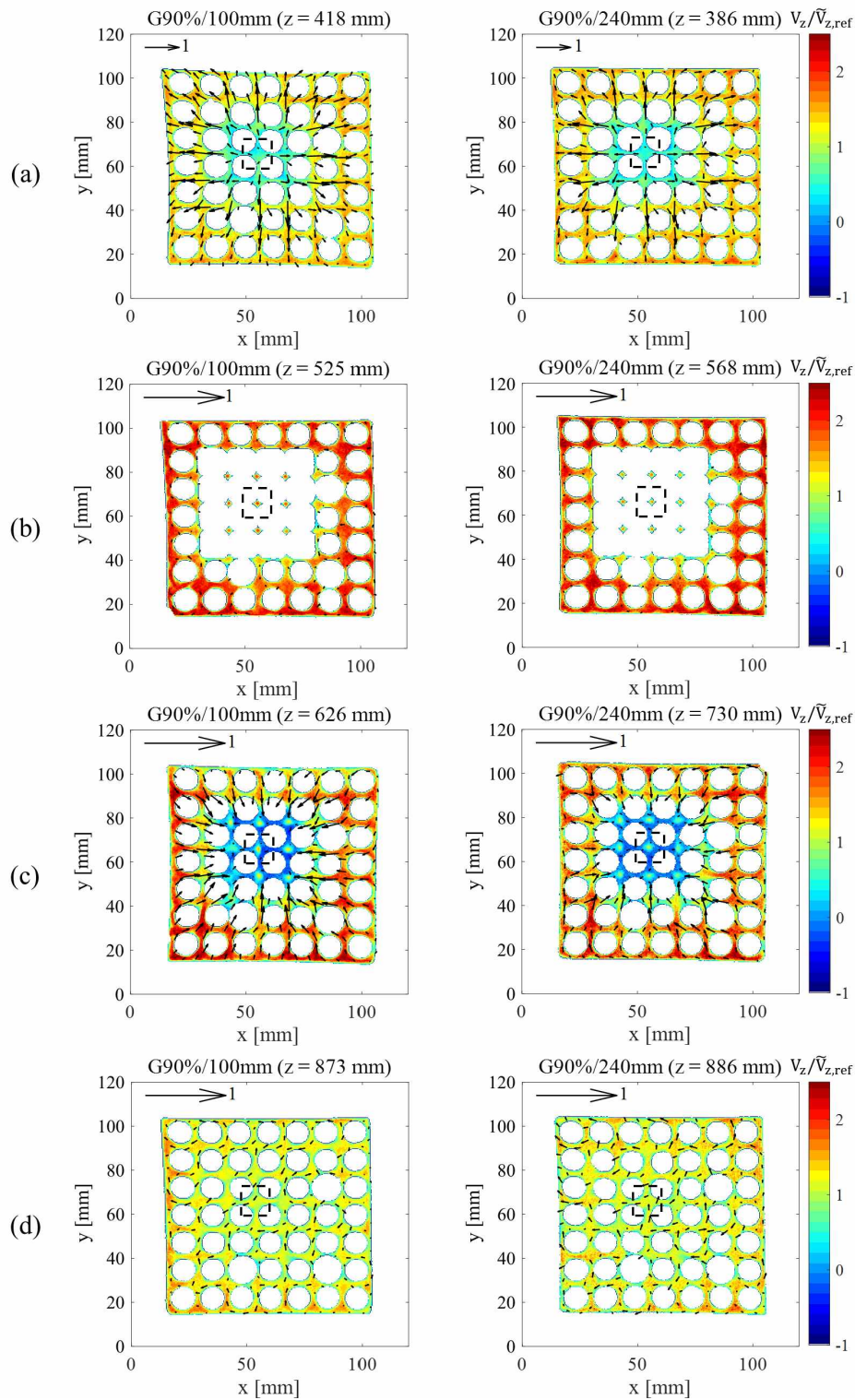
Figure 17: Velocity fields for different bundles comparing the blockage length effect. The sub-channel highlighted by the black box in each bundle was used to trace the profiles in Fig. 18 and to calculate Eq.7.
