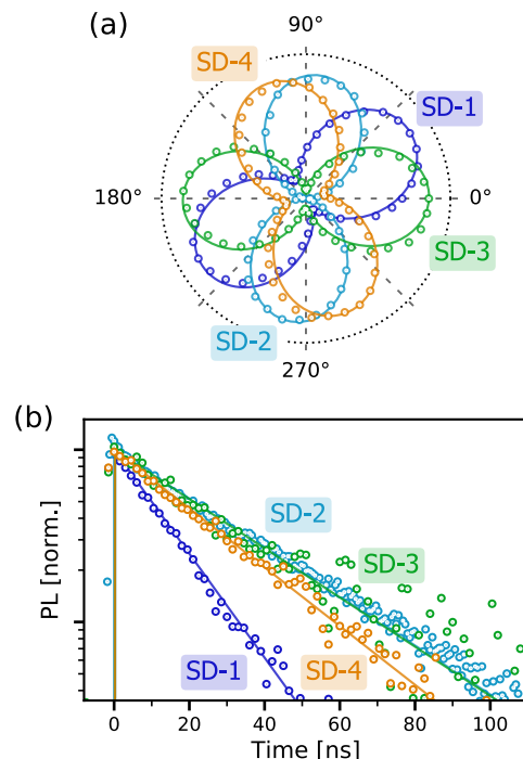
FIG. 3. (a) Emission polarization diagram measured on single defects from families SD-1 to SD-4. The PL signal is recorded while rotating a polarizer in the detection path and corrected from background counts. The 0^\circ and 90^\circ directions match the crystal axes [110] and [\bar{1}\bar{1}0] . Solid lines are fits using a \cos^2(\theta) function. (b) Time-resolved PL decay recorded on the same defects under 50-ps pulse excitation at 532 nm. The excited-state lifetime is extracted by fitting the data with a single exponential function (solid line). Data related to SD-5 and SD-6 defects can be found in SI.
