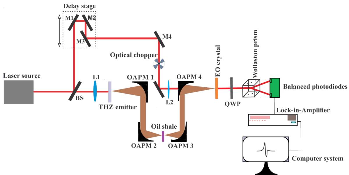
Fig. 2. A typical THz-TDS setup in the transmission mode. BS; Beam Splitter, L1-L2; Lens, M1-M4; Mirrors, OAPM1-OAPM4; Off Axis Parabolic Mirrors, QWP; Quarter Wave Plate.
