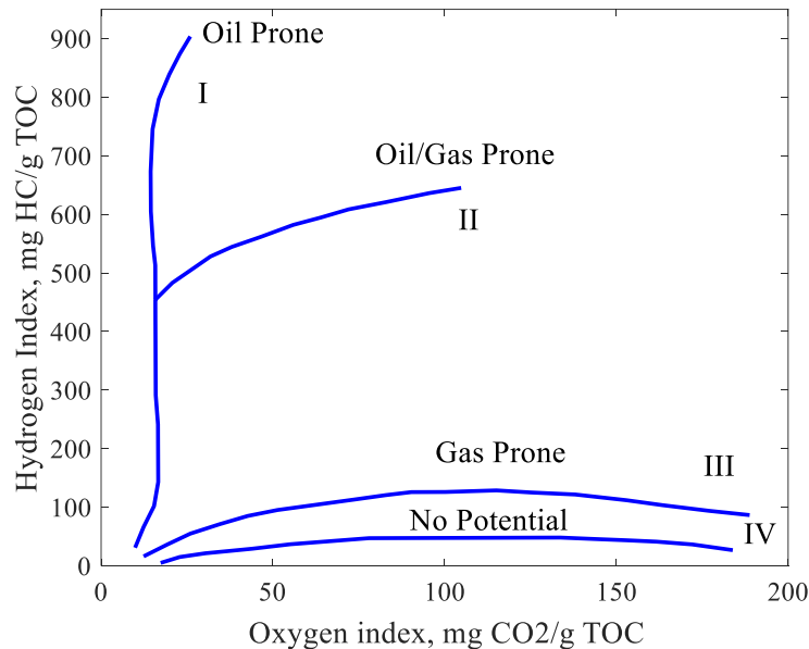
Fig.1. An example of Van-Krevelan diagram for the type I, II, III and IV kerogen.
