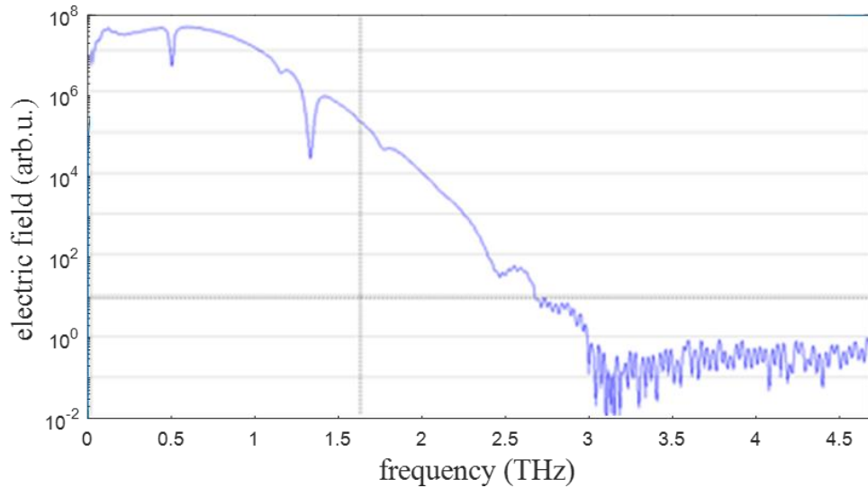
Fig. 4. A Typical spectrum plot from a THz-TDS
