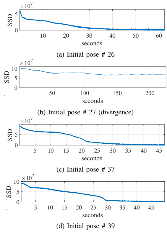
Fig. 7: Evolution of the Sum-of-Squared-Differences cost (SSD) between images brightness during the Defocus-based DVS from several initial poses on the sphere of radius 40 cm.
