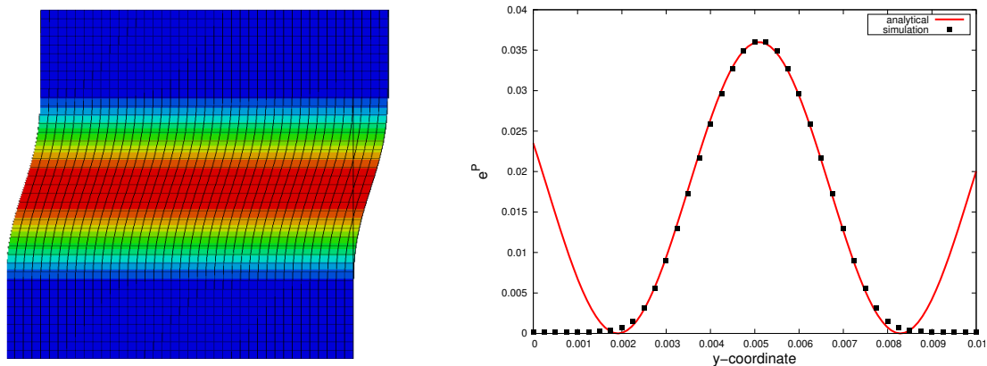
Figure 2. Comparison between numerical and analytical solution for the softening plate. Parameters: B = 10.0 \text{ GPa} , \beta = 500.0 \text{ MPa mm}^2 , H = -500.0 \text{ MPa} , h = 10 \text{ mm} .
