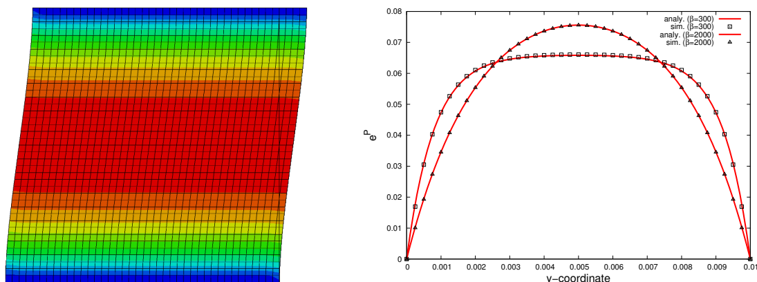
Figure 5. Comparison between numerical and analytical solution for the hardening plate. Parameters: B = 10.0 GPa, \beta = 300.0 MPa mm 2 and 2000.0 MPa mm 2 , H = 500.0 MPa, h = 10 mm.
