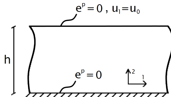
Figure 3. Schematic of the simple glide problem for hardening and perfectly plastic plate: periodic conditions are applied at both ends.
