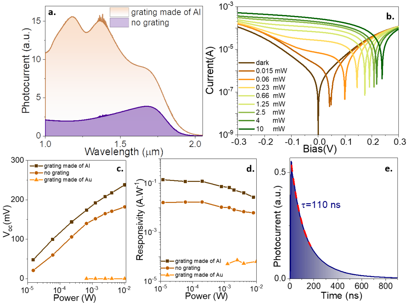
Figure 6 a. Photocurrent spectra for the glass/FTO./HgTe1.7 \mu\text{m} /Hg:Ag 2 Te/Gold stack with and without GMR Al grating. b. IV curves for the glass/FTO:Al-2D grating/HgTe1.7 \mu\text{m} /Hg:Ag 2 Te/Gold stack under different incident power. The illumination is performed with a 1.55 \mu\text{m} laser diode. c. Open circuit voltage of the diode as a function of the incident power without GMR grating and with an Au or Al based grating. Also see Figure S11 for associated IV curves. d. The responsivity of the glass/FTO:Al-2D grating/HgTe1.7 \mu\text{m} /Hg:Ag 2 Te/Gold stack as a function of the incident power using a 1.55 \mu\text{m} laser as source. e. Current as a function of time while the sample has been illuminated by a short (<2 ns) pulse of light (355 nm). Measurements are conducted under a 0 V bias operation and in ambient conditions.
