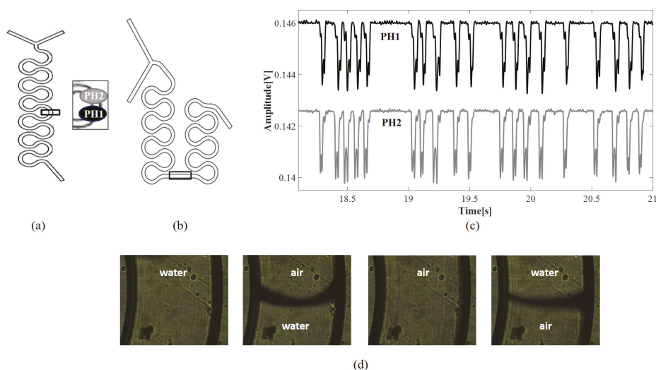
Figure 2. (a) the geometry of the serpentine channel of 320 \mu\text{m} (labelled as G-320); (b) the geometry of serpentine channel of 640 \mu\text{m} (labelled as G-640); (c) an example of the trends of the signals acquired by the two photo-diodes \{ph1, ph2\} in G-320 in the experiment with an input flow rate F = 0.3 \text{ mL/min} . The two rectangles in G-320 and G-640 point out the investigation areas where the two-photo-diodes are placed; (d) a frame sequence related to the slug passage acquired by the CCD.
