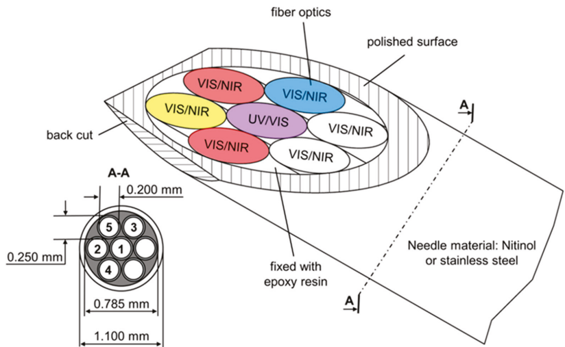
Figure 13. Needle probe for multispectral backscattering measurements. Ultraviolet (UV), visible (VIS), NIR, and fluorescence measurements are possible. The needle is optimized for tissue penetration with a front and back cut [13].
