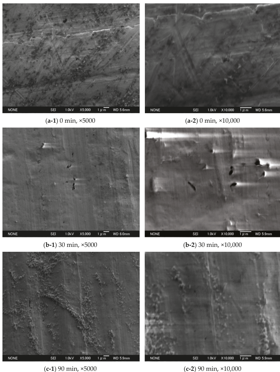
Figure 1. Scanning electron microscope (SEM) images of the anodic oxide films on the sample surfaces: (a) 0 min; (b) 30 min; and (c) 90 min with the magnification of (1) \times 5000 ; and (2) \times 10,000 .
