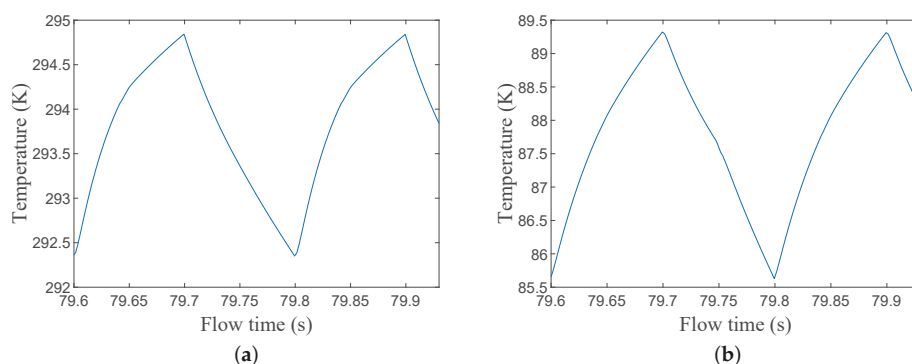
Figure 11. (a) Temperature changes during cooling and heating periods at the regenerator's hot end. (b) Temperature changes during cooling and heating periods at the regenerator's cold end.
