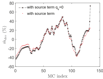
Figure 10. Flow maldistribution with and without source term q_v for counterflow configuration with \dot{m}_f = 2.5 kg/s.
