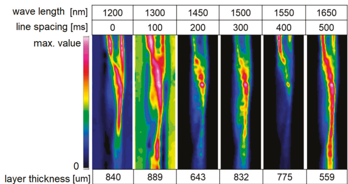
Figure 7. Near-infrared (NIR) measurement on water strands at all different wavelengths 274 × 142 mm (220 × 220 DPI), water glycerin [21].
