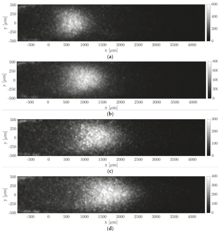
Figure 18. MTV acquisitions of helium–acetone flow with \chi = 20\% : (a) \Delta t = 20 \mu s, \Delta t_{gate} = 500 ns, p_m = 920 Pa, and \Delta p = 1092.7 Pa; (b) \Delta t = 30 \mu s, \Delta t_{gate} = 1000 ns, p_m = 920.3 Pa, and \Delta p = 1093.4 Pa; (c) \Delta t = 40 \mu s, \Delta t_{gate} = 500 ns, p_m = 919.1 Pa, and \Delta p = 1091.8 Pa; and (d) \Delta t = 50 \mu s, \Delta t_{gate} = 1000 ns, p_m = 919.1 Pa, and \Delta p = 1090.7 Pa. The recording parameters used are: N_l = 100 , N_i = 20 , and G = 100\% . The acquisitions are made with a 4 \times 4 binning. The laser pulse energy was varying between 80 and 100 \mu J.
