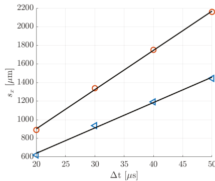
Figure 20. Mean molecular displacement \bar{s}_x in helium flow at delays \Delta t = 20, 30, 40 , and 50 \mu\text{s} : (O) data at 1.6 kPa; ( \triangleleft ) data at 920 Pa. The black solid line represents the linear interpolation of the MTV data, which provides an average velocity \bar{u}_{MTV} = 42.2 \text{ m/s} for the data at 1.6 kPa and \bar{u}_{MTV} = 27.28 \text{ m/s} for the data at 920 Pa.
