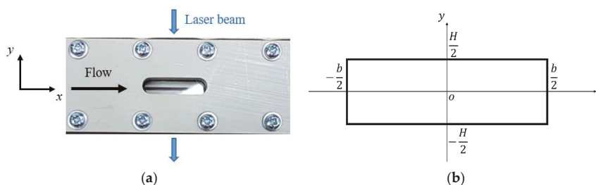
Figure 3. In (a), a global view of the test section along the channel from the point of the CCD camera. The blue arrows indicate the optical access for the laser beam and the black arrow shows the gas flow direction. In (b), a sketch of the channel cross-section along with the adopted Cartesian coordinate system.
