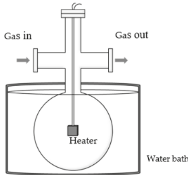
Figure 2. A schematic of the experimental setup.
