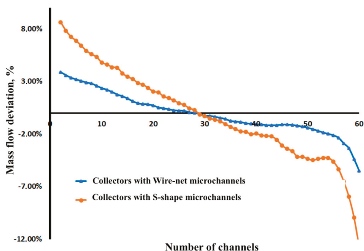
Figure 5. Mass flow rate deviation of perturbators based on Reduced Order Model (ROM).
