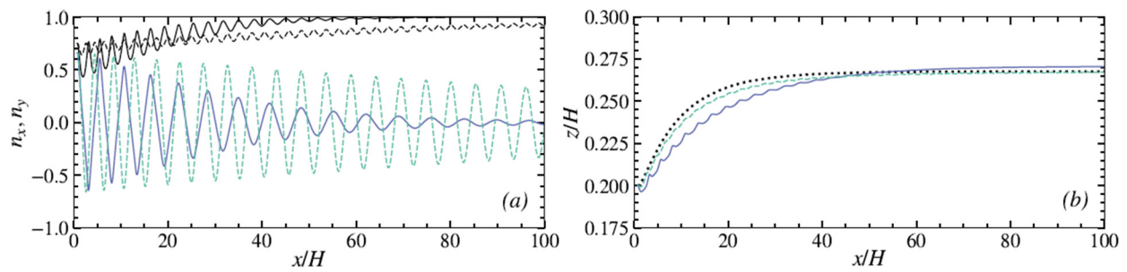
Figure 10. (a) x -components (colored curves) and y -components (black curves) of the orientation vector of an oblate and (b) trajectories for spheroids with \kappa = 0.15 and \lambda = 0.5 (solid), 0.8 (dashed), and 1 (dotted) (reprinted from [17], with the permission of AIP Publishing).
