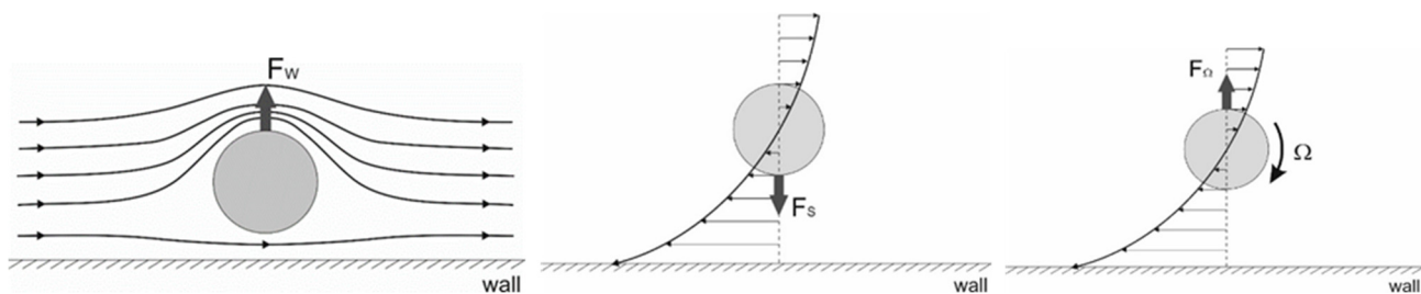
Figure 2. Illustration of the wall-induced lift force F_w , the shear-induced lift force F_s , and the rotation-induced lift force F_\Omega .
