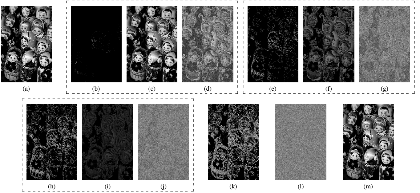
Fig. 7: Illustration of our proposed recursive method: a) Original Dolls image I of 666 \times 1,000 pixels, b) PE location map associated to the 1 st bit-plane I_0^{[0]} (MSB-plane), number of errors = 1,628 (0.2%), c) Adapted image I_1^{[0,7]} after PE consideration, d) Image I_{E-DH}^{[0]} + I_1^{[1,7]} composed of the marked encrypted 1 st bit-plane and the 7 least significant bit-planes of (c), payload = 0.9804 bpp , e) PE location map associated with the 2 nd bit-plane I_1^{[1]} , number of errors = 29,324 (4.4%), f) Adapted image I_2^{[1,7]} after PE consideration, g) Image I_{E-DH}^{[0,1]} + I_2^{[2,7]} composed of the marked encrypted 1 st and 2 nd bit-planes and the 6 least significant bit-planes of (f), payload = 1.6722 bpp (+0.6918 bpp ), h) PE location map associated with the 3 rd bit-plane I_2^{[2]} , number of errors = 77,094 (11.58%), i) Adapted image I_3^{[2,7]} after PE consideration, j) Image I_{E-DH}^{[0,2]} + I_3^{[3,7]} composed of the marked encrypted 1 st , 2 nd and 3 rd bit-planes and the 5 least significant bit-planes of (i), payload = 1.9777 bpp (+0.3055 bpp ), k) PE location map associated with the 4 th bit-plane I_3^{[3]} , number of errors = 144,014 (21.63%), l) Image I_{E-DH} after encryption using all bit-planes and data embedding in the 1 st , 2 nd and 3 rd bit-planes, final payload = 1.9777 bpp , m) Reconstructed original image I , PSNR \rightarrow +\infty , SSIM = 1.
