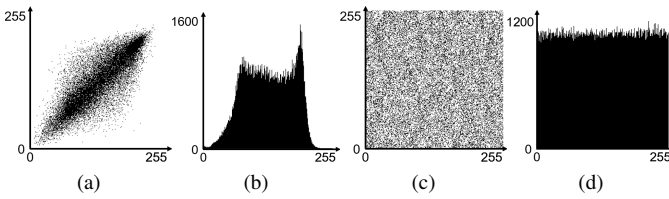
Fig. 10: Statistical representations (correlation and histogram) for the original Baboon image and the associated marked encrypted image obtained with our method illustrated Fig. 9.a: a) Horizontal correlation in the original image, b) Histogram of the original image, c) Horizontal correlation in the marked encrypted image (Fig. 9.a), d) Histogram of the marked encrypted image (Fig. 9.a).
