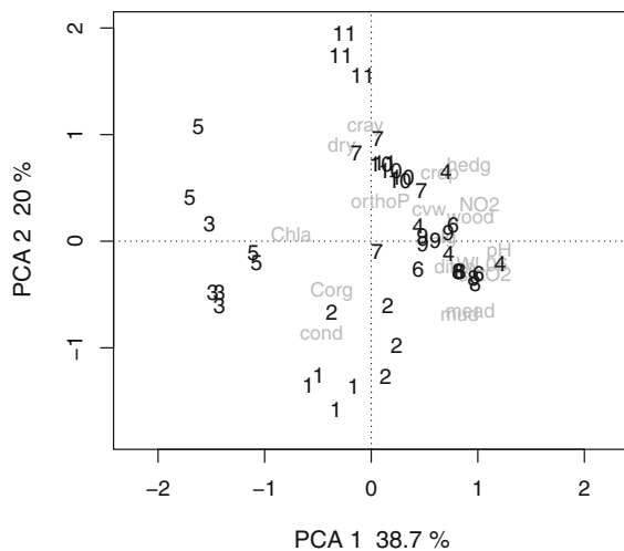
Fig. 3 Unweighted scaled PCA based on all environmental variables for all 11 sites, over four years. Sites are indicated according to their scores on the first two components PCA1 and PCA2 for each year and variable
