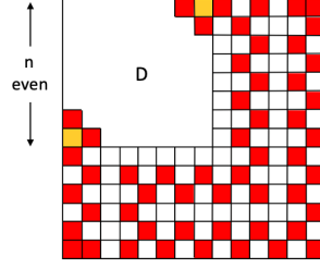
Figure 3: Illustration of Proposition 12. The vertices are depicted as small squares (with most vertices inside G_{n \times n} as well as their status omitted). Initially infected (resp., not infected) vertices of D'' are red (resp., white). Orange vertices are the ones that are initially infected in D but not in D'' .
