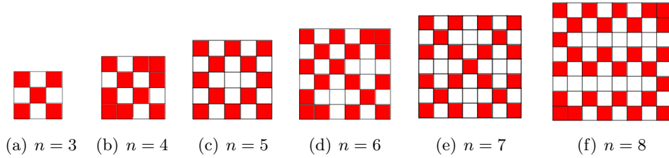
Figure 1: Some instances of minimum lethal sets in G_{n \times n} when r = 3 .
