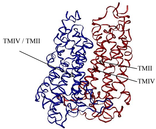
Dimer II-IV/II-IV
