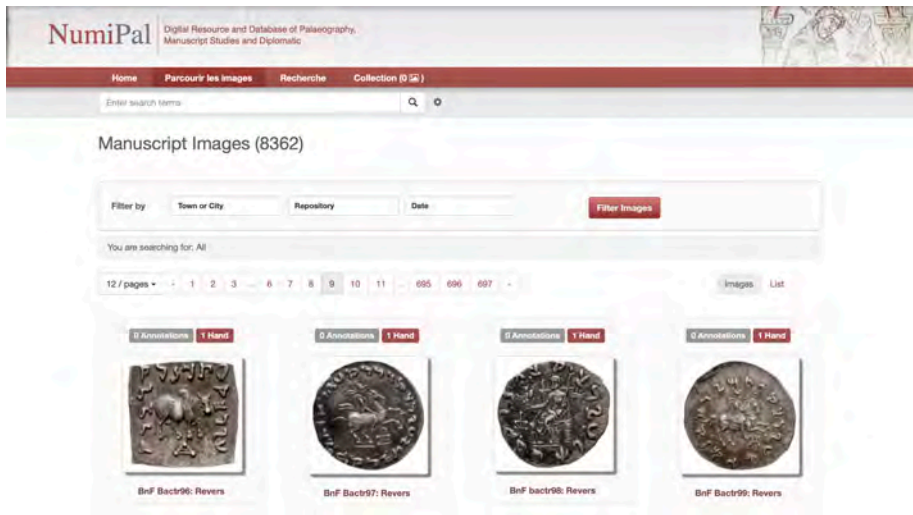
FIGURE 3. NumiPal website
