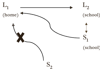
FIGURE 4. A schematic showing how the script of a language learned for educational purposes becomes S_1 and will therefore tend to be adopted for a previously unwritten L_1 .
