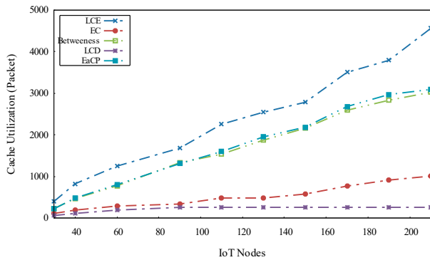
Fig. 3: Cache Utilization.
