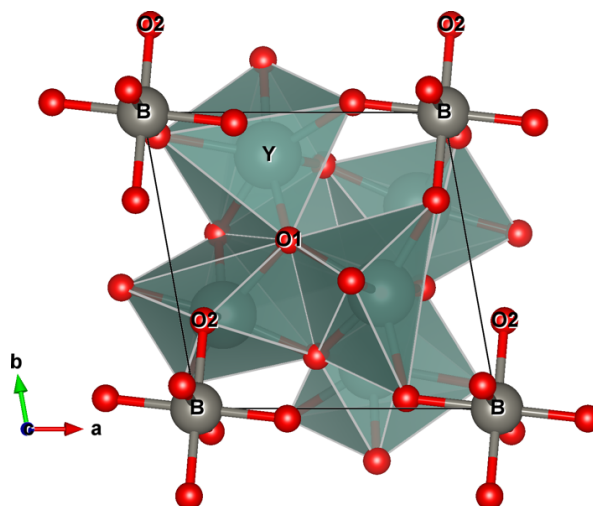
Fig. 1 Left panel: Atomic position of the fully relaxed structure of Y_6WO_{12} obtained by DFT calculation (B=W). Right panel: representation of the primitive rhombohedral trigonal structure.
