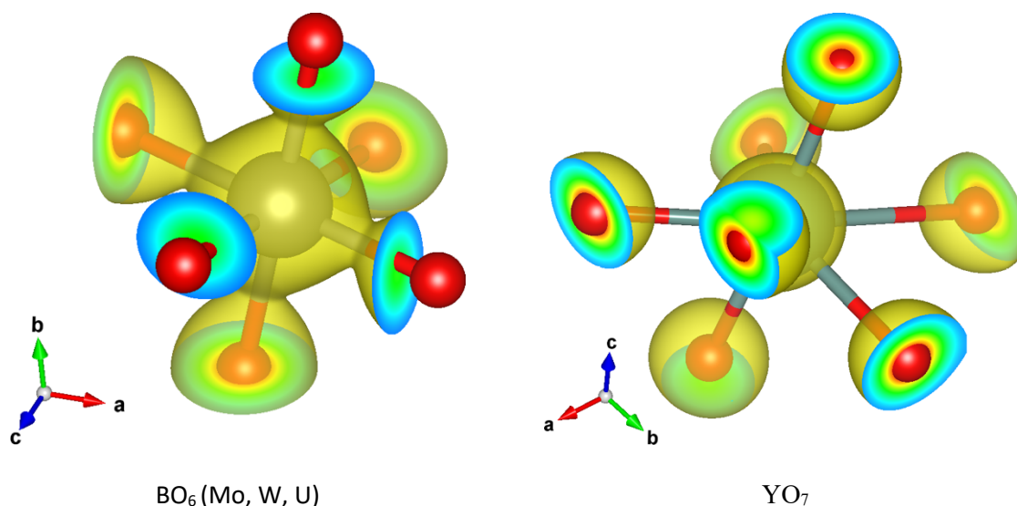
Fig. 2 Contour maps showing the charge density distributions for the two polyhedra in the ordered \delta -phase structures of Y_6MoO_{12} , Y_6WO_{12} , and Y_6UO_{12} .
